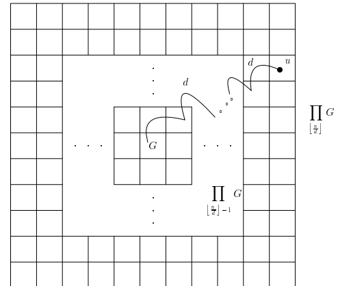
Fig. 7. \prod_{\lfloor \frac{n}{d} \rfloor} G \subseteq \mathcal{M}_n(G) .
