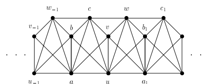
Fig. 18. Average-measurable graph with d_\infty(G) = 5 .
