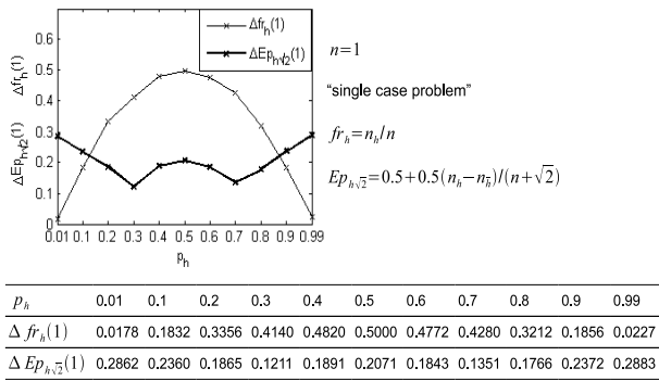
Fig. 19. Diagram of the average, absolute, one-sample item error \Delta_{fr_h}(1) and \Delta_{Ep_{h\sqrt{2}}}(1) of the frequency estimator fr_h and of the completeness estimator Ep_{h\sqrt{2}} from estimation of different 11 probabilities p_h for n = 1 (single case problem). The results are averaged for 1000 experiments.
