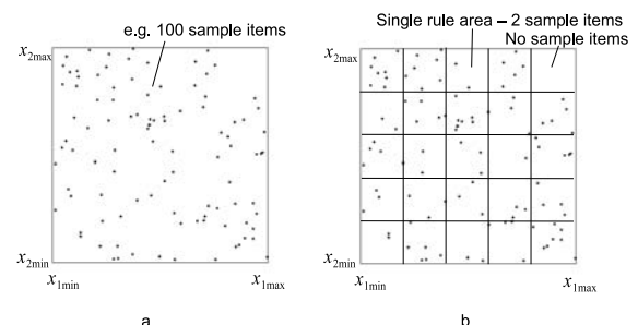
Fig. 1. Example illustrating a small number of sample items in the problem of probability estimation of rules detected with rough set theory or fuzzy set theory: sample items in the whole input space (a), sample items in the subspaces of single rules (regular input-space partition) (b).
