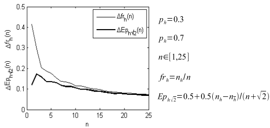
Fig. 15. Diagram of the average, absolute errors \Delta_{fr_h}(n) and \Delta_{Ep_{h,\sqrt{2}}}(n) of the frequency estimator fr_h and the completeness estimator Ep_{h,\sqrt{2}} for estimation of antonym probabilities p_h = 0.3 and p_h = 0.7 for sample item numbers n \in [1, 25] . The results are averaged for 1000 experiments.
