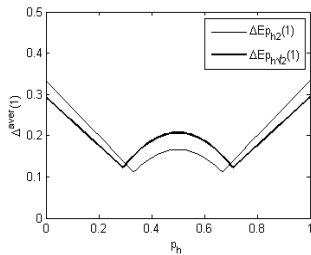
Fig. 26. Comparison of the mean absolute errors made by the two compared estimators, the E_{p_{h\sqrt{2}}} estimator (bold line) and the Cestnik–Laplace estimator E_{p_{h2}} (thin line) in estimation of probabilities p_h \in [0, 1] on the basis of only one sample item (simple case problem).
