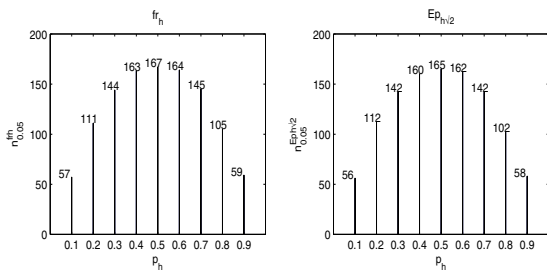
Fig. 24. Approximate, minimal sample item numbers n_{0.05}^{f_{r_h}} and n_{0.05}^{E_{p_h\sqrt{2}}} necessary for identification of various probabilities p_h with the use of the frequency estimator f_{r_h} and the completeness estimator E_{p_h\sqrt{2}} with the absolute error less than 0.05. The results are averaged for 1000 experiments for each p_h -value.
