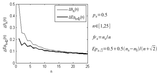
Fig. 12. Diagram of the average, absolute, estimation error \Delta_{fr_h}(n) of the frequency estimator fr_h and of the error \Delta_{Ep_{h\sqrt{2}}}(n) of the completeness estimator Ep_{h\sqrt{2}} for small numbers of sample items n \in [1, 25] calculated on the basis of 1000 experiments with 10000 numbers in each experiment. The estimated probability was p_h = 0.5 .
