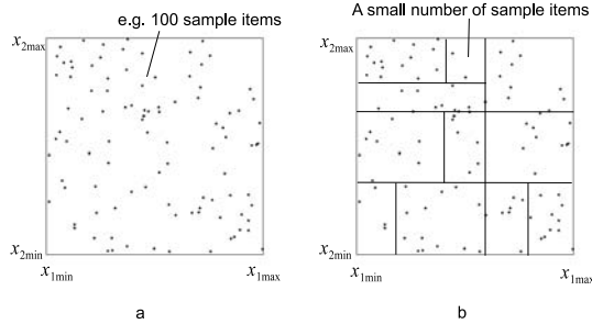
Fig. 2. Illustration of a small number of sample items occurring in influence subspaces of particular rules detected with the method of decision trees: sample items in the whole input space (a), sample items in subspaces of single rules (non-regular input space partition) (b).
