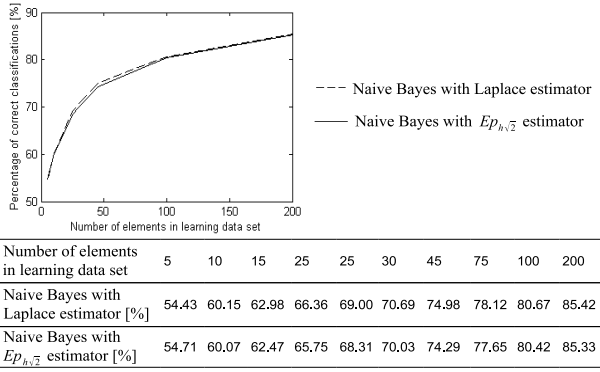
Fig. 28. Percentage of correct classifications of examples from testing data set, depending on the number of elements in the learning data set, using naive Bayes classifiers with Laplace estimator and with the Ep_{h\sqrt{2}} estimator.
