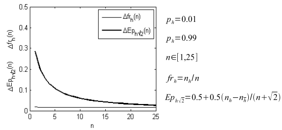
Fig. 18. Diagram of the average, absolute estimation errors \Delta_{fr_h}(n) and \Delta_{Ep_{h,\sqrt{2}}}(n) of probabilities p_h = 0.01 and p_h = 0.99 (practical certainty) made by the frequency estimator fr_h and the completeness estimator Ep_{h,\sqrt{2}} . The results are averaged for 1000 experiments.
