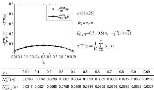
Fig. 23. Diagram of the average, absolute error \Delta_{f_{r_h}}^{aver}(n) and \Delta_{E_{p_h\sqrt{2}}}^{aver}(n) of the frequency estimator f_{r_h} and the completeness estimator E_{p_h\sqrt{2}} from estimation of 11 different p_h -probabilities for sample item numbers n \in [16, 25] . The results are averaged for 1000 experiments for each p_h -value.
