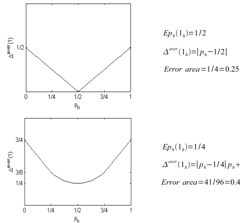
Fig. 9. Cross-sections of the average, one-sample item error function \Delta^{aver}(1) = f(p_h, Ep_h(1_h)) from Fig. 6 for estimate values Ep_h(1_h) = 1/2 and Ep_h(1_h) = 1/4 assigned to one sample item 1_h confirming the hypothesis h .
