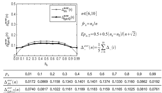
Fig. 21. Diagram of the average, absolute error \Delta_{aver}^n(fr_h) and \Delta_{aver}^n(Ep_{h\sqrt{2}}) of the frequency estimator fr_h and the completeness estimator Ep_{h\sqrt{2}} for estimation of 11 different probabilities p_h from sample item numbers n \in [6, 10] . The results are averaged for 1000 experiments for each p_h -value.
