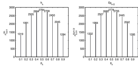
Fig. 25. Approximate, minimal sample item numbers n_{0.01}^{f_{r_h}} and n_{0.01}^{E_{p_h\sqrt{2}}} necessary for identification of various probabilities p_h with the use of the frequency estimator f_{r_h} and the completeness estimator E_{p_h\sqrt{2}} with the absolute error less than 0.01. The results are averaged for 1000 experiments for each p_h -value.
