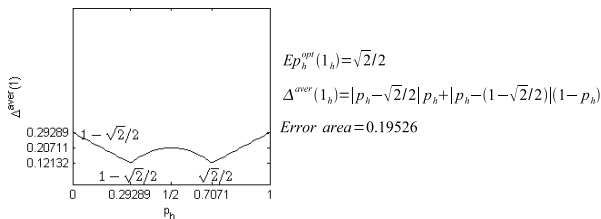
Fig. 11. Cross-section of the function \Delta^{aver}(1) of the absolute, average, one-sample item error for the optimal one-sample item estimate Ep_h^{opt}(1_h) = \sqrt{2}/2 .
