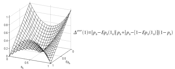
Fig. 6. Functional surface of the complete dependence \Delta^{aver}(1) = f(p_h, Ep_h(1_h)) of the average absolute error of one-sample item probability estimation.
