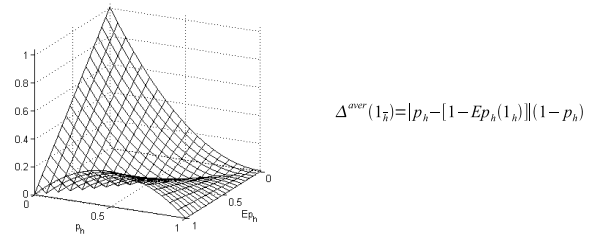
Fig. 5. Functional surface of the dependence \Delta^{aver}(1_{\bar{h}}) = f(p_h, Ep_h(1_h)) of the second component of the whole single-sample item error \Delta^{aver}(1) of probability estimation generated by sample items 1_{\bar{h}} , negating the hypothesis h .
