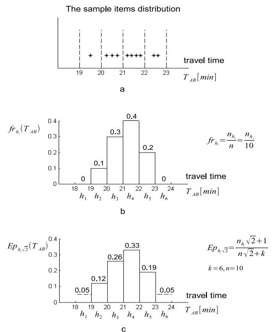
Fig. 29. Distribution of measurement sample items of the travel time T_{AB} [min] between points A and B , histogram of travel time probability determined with the frequency estimator fr_{h_i} = n_{h_i}/n (b), histogram determined on the basis of the optimal completeness estimator Ep_{h_i\sqrt{2}} (c).
