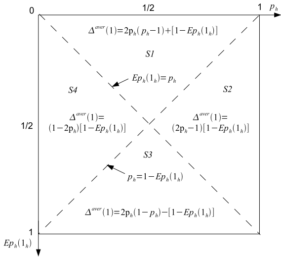
Fig. 10. Four sectors S1 – S4 in the space of independent variables p_h and Ep_h(1_h) of the one-sample item, average error function \Delta^{aver}(1) = f(p_h, Ep_h(1_h)) .
