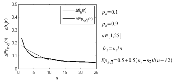
Fig. 17. Diagram of average, absolute errors \Delta_{fr_h}(n) and \Delta_{Ep_{h,\sqrt{2}}}(n) of the frequency estimator fr_h and of the completeness estimator Ep_{h,\sqrt{2}} for estimation of probabilities p_h = 0.1 and p_h = 0.9 for sample item numbers n \in [1, 25] . The results are averaged for 1000 experiments.
