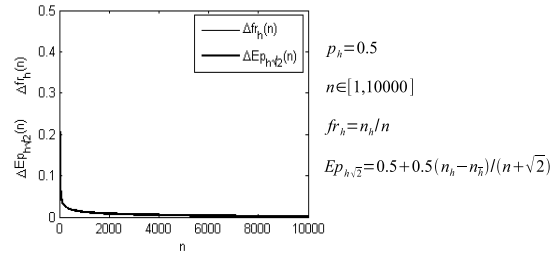
Fig. 13. Diagram of the average, absolute error \Delta_{fr_h}(n) of the frequency estimator fr_h and of the error \Delta_{Ep_{h\sqrt{2}}}(n) of the completeness estimator Ep_{h\sqrt{2}} for full experiment series n \in [1, 10000] sample items. The result is averaged for 1000 experiments.
