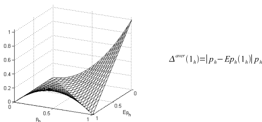
Fig. 4. Functional surface of the dependence \Delta^{aver}(1_h) = f(p_h, Ep_h(1_h)) of the first component of the total error \Delta^{aver}(1) representing weighted estimation errors of sample items 1_h confirming the hypothesis h .
