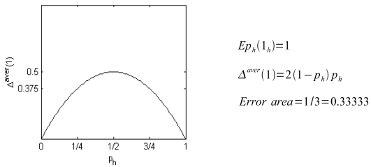
Fig. 7. Cross section of the average, single-sample item error \Delta^{aver}(1) from Fig. 6 for the probability estimate Ep_h(1_h) = 1 that corresponds to the estimate calculated by the frequency estimator fr_h = n_h/n .
