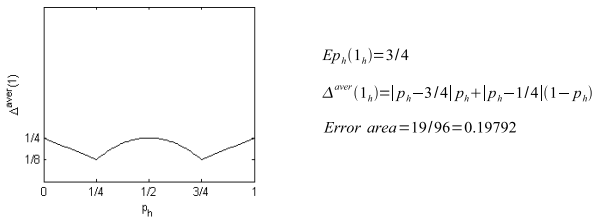
Fig. 8. Cross section of the average, one-sample item error \Delta^{aver}(1) function from Fig. 6 for the estimate value Ep_h(1_h) = 3/4 assigned to one sample item 1_h confirming the hypothesis h .
