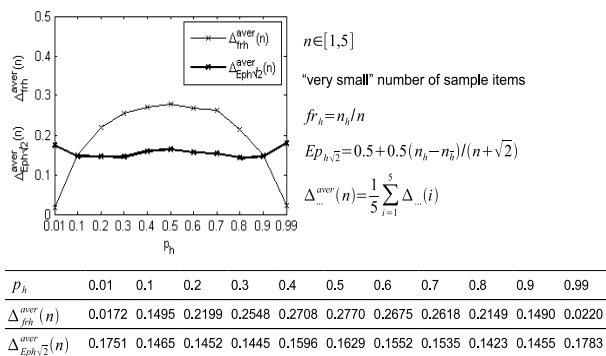
Fig. 20. Diagram of the average, absolute error \Delta_{aver}^n(fr_h) and \Delta_{aver}^n(Ep_{h\sqrt{2}}) of the frequency estimator fr_h and the completeness estimator Ep_{h\sqrt{2}} for estimation of 11 different probabilities p_h on the basis of sample item numbers n \in [1, 5] . The results are averaged for 1000 experiments for each p_h -value.
