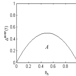
Fig. 3. Dependence of the average error \Delta^{aver}(1) of the one-sample item conclusion concerning the real value p_h of hypothesis probability for the frequency estimator fr_h .
