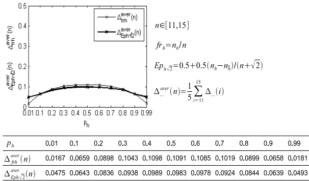
Fig. 22. Diagram of the average, absolute error \Delta_{f_{r_h}}^{aver}(n) and \Delta_{E_{p_h\sqrt{2}}}^{aver}(n) of the frequency estimator f_{r_h} and the completeness estimator E_{p_h\sqrt{2}} from estimation of 11 different p_h -probabilities for sample item numbers n \in [11, 15] . The results are averaged for 1000 experiments for each p_h -value.
