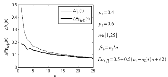
Fig. 14. Diagram of the average, absolute errors \Delta_{fr_h}(n) and \Delta_{Ep_{h\sqrt{2}}}(n) of the frequency estimator fr_h and of the completeness estimator Ep_{h\sqrt{2}} for estimation of the antonym probabilities p_h = 0.4 and p_h = 0.6 for sample item numbers n \in [1, 25] . The diagram shows the results averaged for 1000 experiments.
