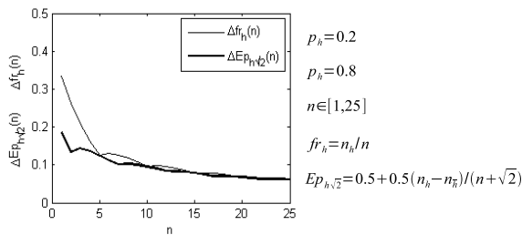
Fig. 16. Diagram of average, absolute errors \Delta_{fr_h}(n) and \Delta_{Ep_{h,\sqrt{2}}}(n) of the frequency estimator fr_h and of the completeness estimator Ep_{h,\sqrt{2}} for estimation of antonym probabilities p_h = 0.2 and p_h = 0.8 for sample item numbers n \in [1, 25] . The results are averaged for 1000 experiments.
