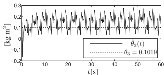
Fig. 14. Time evolution of the estimated parameter \hat{\theta}_3(t) for Test 2.
