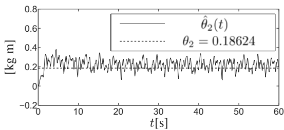
Fig. 6. Time evolution of the estimated parameter \hat{\theta}_2(t) for Test 1.
