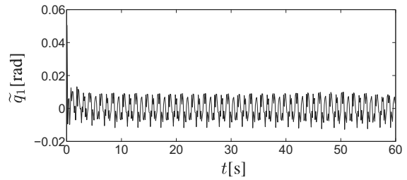
Fig. 8. Time evolution of the tracking error for Joint 1 denoted by \tilde{q}_1(t) for Test 2.
