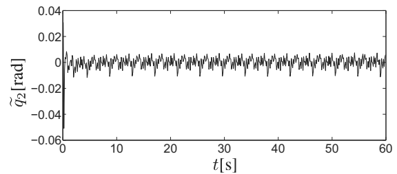
Fig. 9. Time evolution of the tracking error for Joint 2 denoted by \tilde{q}_2(t) for Test 2.
