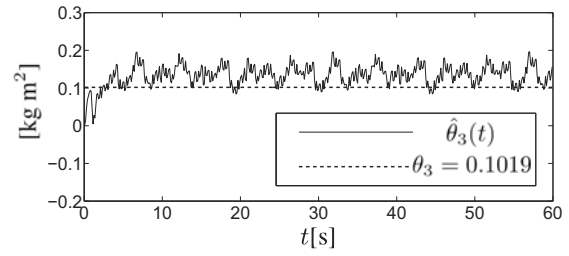
Fig. 7. Time evolution of the estimated parameter \hat{\theta}_3(t) for Test 1.
