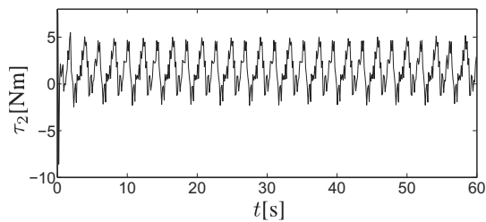
Fig. 11. Time evolution of the torque applied for Joint 2 denoted by \tau_2(t) for Test 2.
