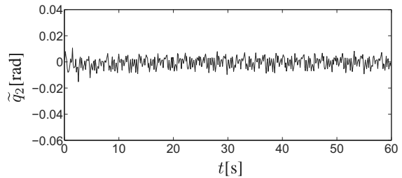
Fig. 2. Time evolution of the tracking error for Joint 2 denoted by \tilde{q}_2(t) for Test 1.
