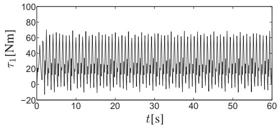
Fig. 3. Time evolution of the applied torque for Joint 1 denoted by \tau_1(t) for Test 1.
