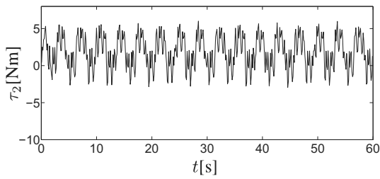
Fig. 4. Time evolution of the torque applied for Joint 2 denoted by \tau_2(t) for Test 1.
