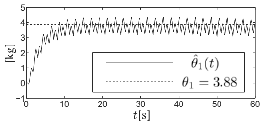
Fig. 12. Time evolution of the estimated parameter \hat{\theta}_1(t) for Test 2.
