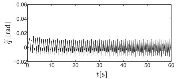
Fig. 1. Time evolution of the tracking error for Joint 1 denoted as \tilde{q}_1(t) for Test 1.
