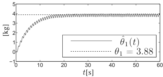
Fig. 5. Time evolution of the estimated parameter \hat{\theta}_1(t) for Test 1.
