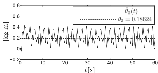
Fig. 13. Time evolution of the estimated parameter \hat{\theta}_2(t) for Test 2.
