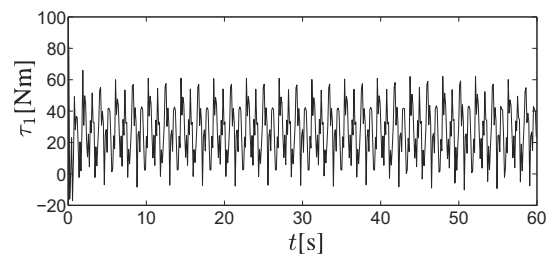
Fig. 10. Time evolution of the torque applied for Joint 1 denoted by \tau_1(t) for Test 2.
