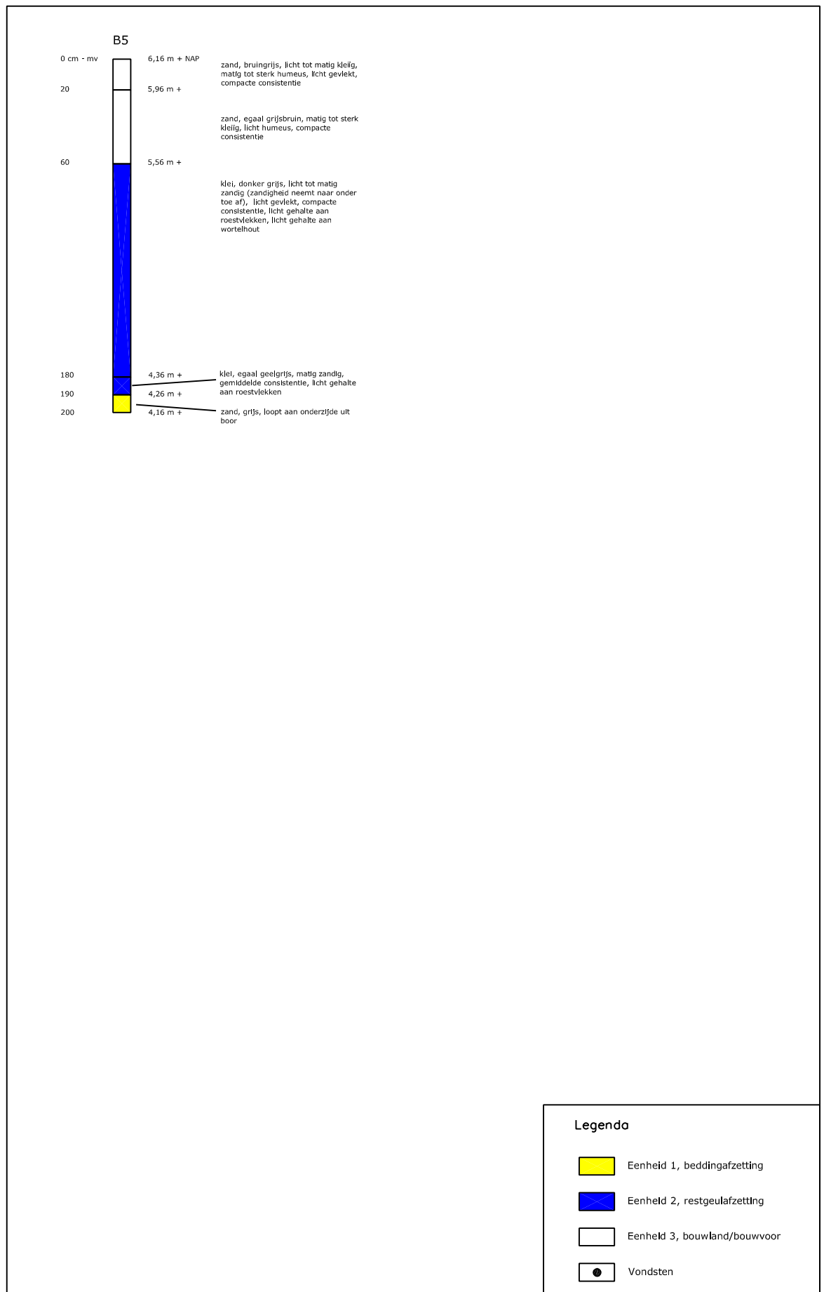
Afb. 5b: Boorstaten, boring 5.
