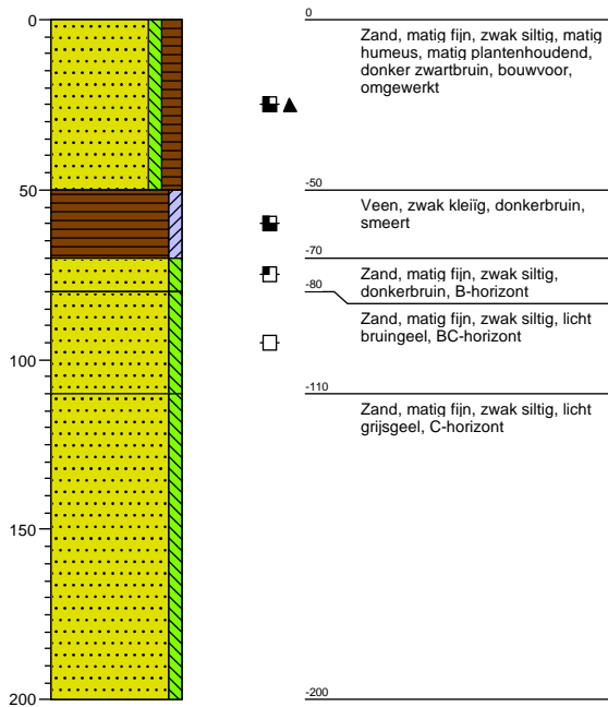
Boring: 7
