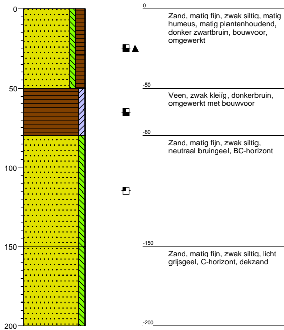
Boring: 5
