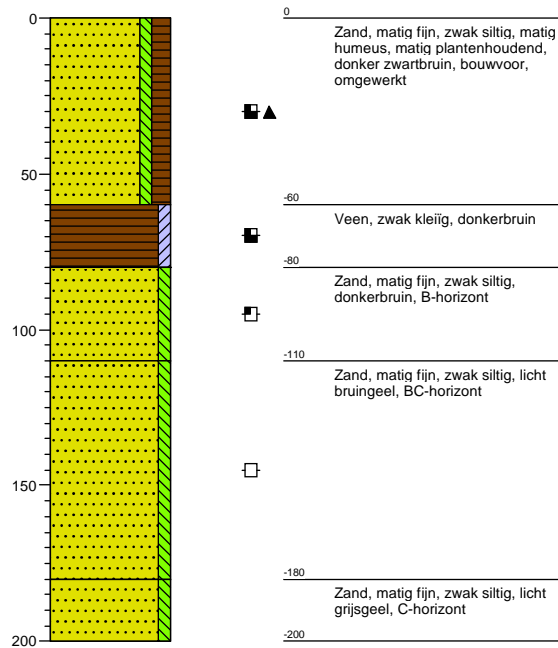
Boring: 8
