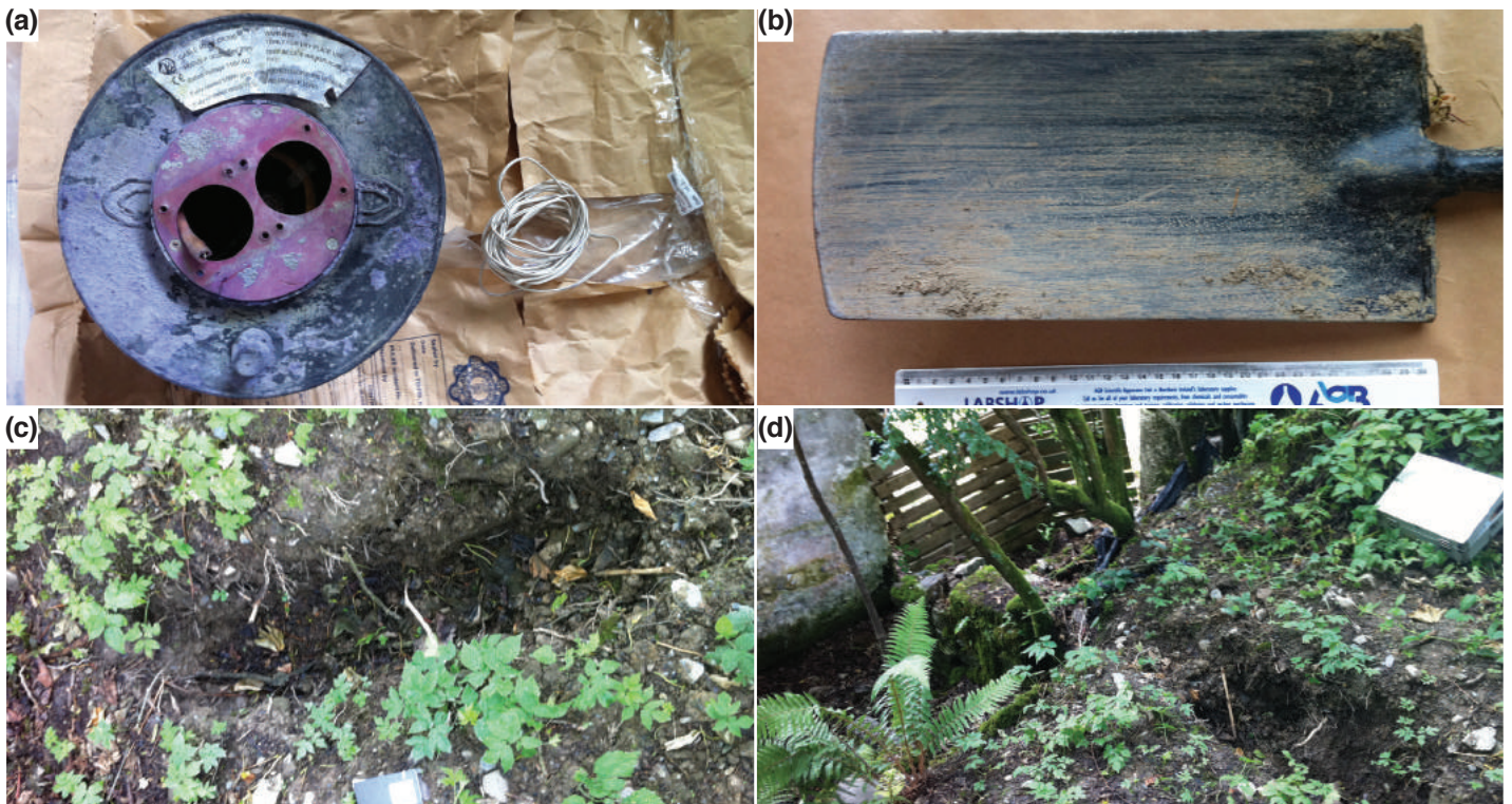
Figure 30.1. (a) Suspected command wire seized from the suspects' vehicle. (b) Soil/mud-encrusted spade that was used for PXRf analysis. (c) Trench in County Derry–Londonderry where the mortar tube was located. (d) The trench that contained the two mortar rounds.
