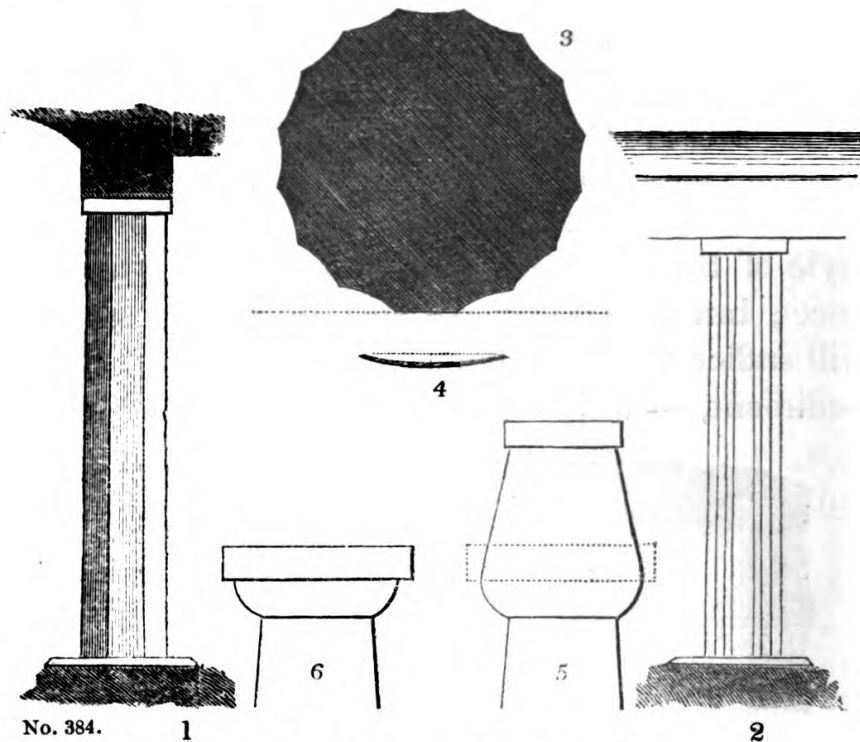
No. 384. 1 Fig. 1. Columns in the portico of the northern grottos of Beni Hassan. 2. Columns of the interior. 3. Horizontal section of fig. 2., showing the grooves. 4. One of the grooves on a larger scale. 5. An Egyptian capital, which seems to have been the origin of the Doric : fig. 6.
