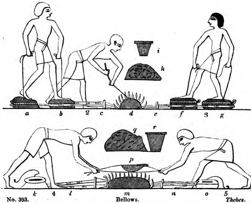
No. 393. Bellows. Thebes. a, b, k, o , the leather case. c, e, l, n , the pipes conveying the wind to the fire. d, m , the fire. h, q , charcoal. k and o are raised as if full of air.
