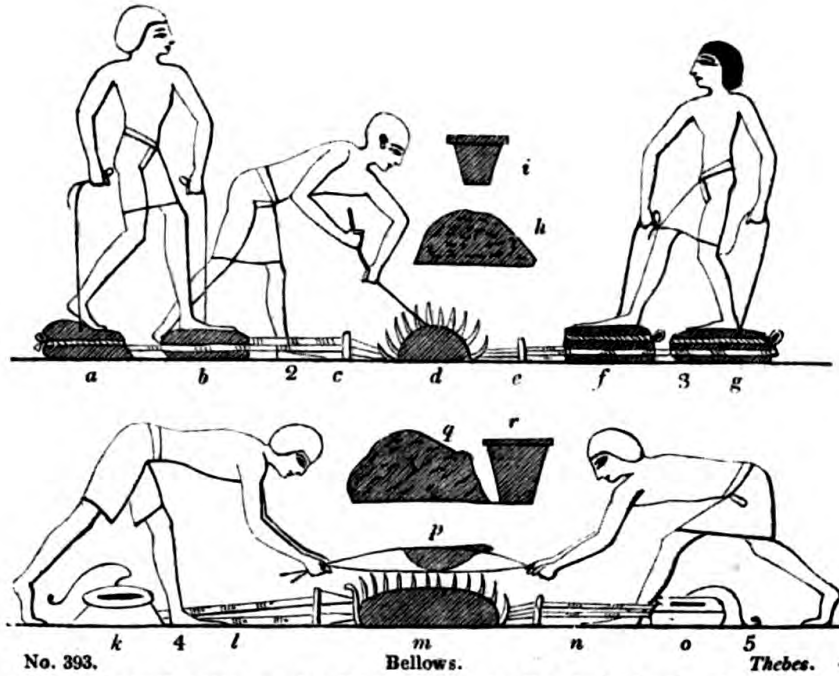
No. 393. k 4 l m n o 5 Thebes . a, b, k, o , the leather case. c, e, l, n , the pipes conveying the wind to the fire. d, m , the fire. h, q , charcoal. k and o are raised as if full of air.
