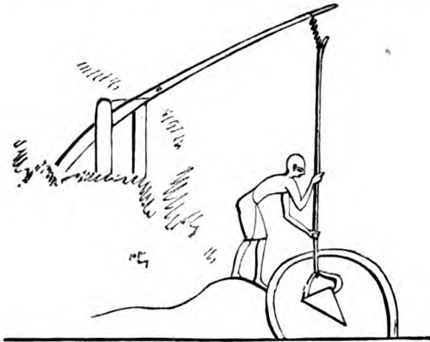
No. 75. Shadóof for watering the lands. Thebes.
