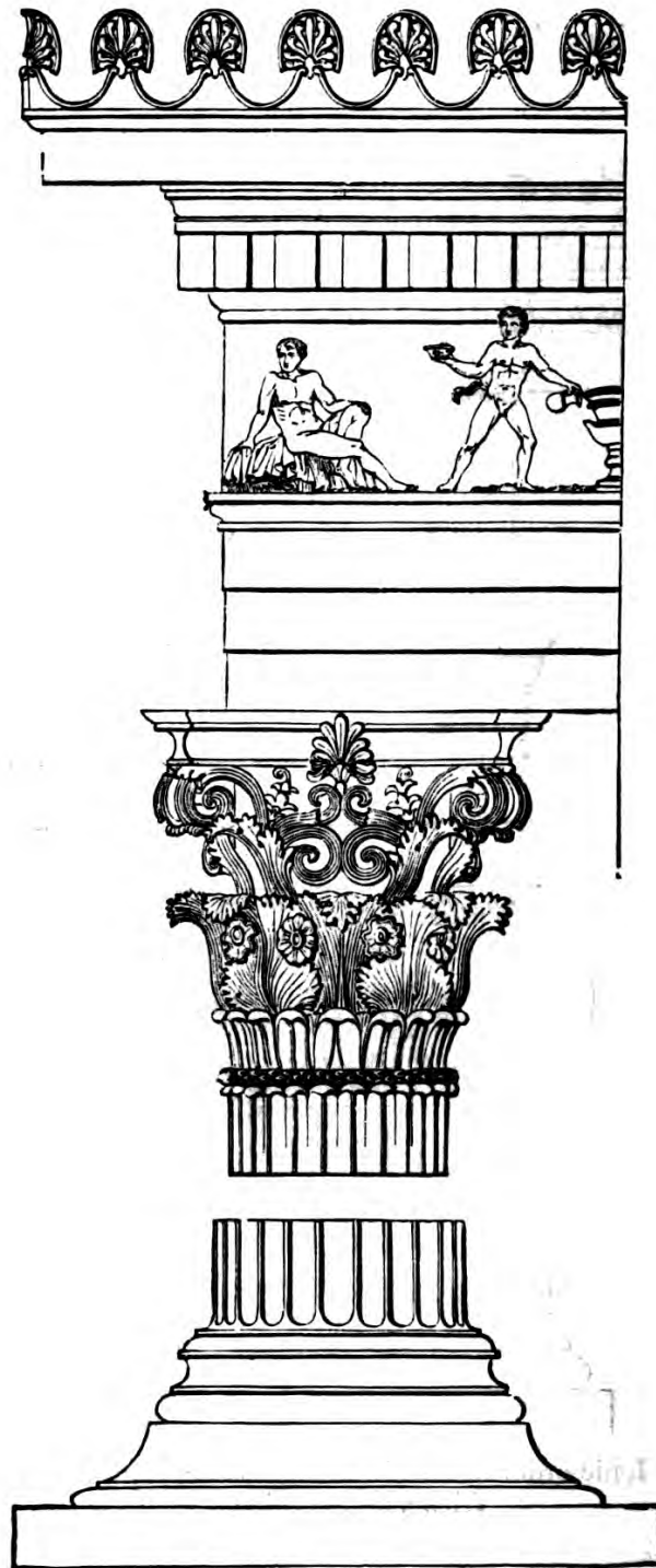
Fig. 136. Corinthian order : monument of Lysicrates, Athens.
