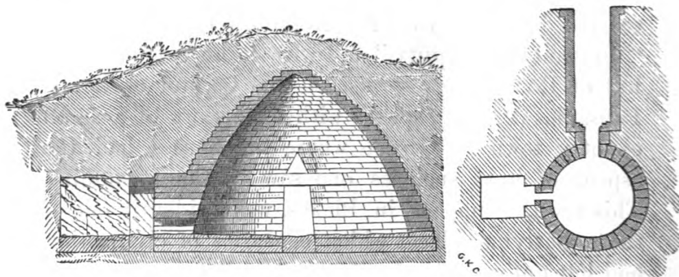
Fig. 128. Tomb of Agamemnon (?) at Mycenæ.
