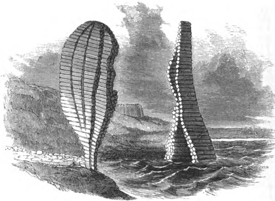
REMAINS OF BASALTIC DYKES.
