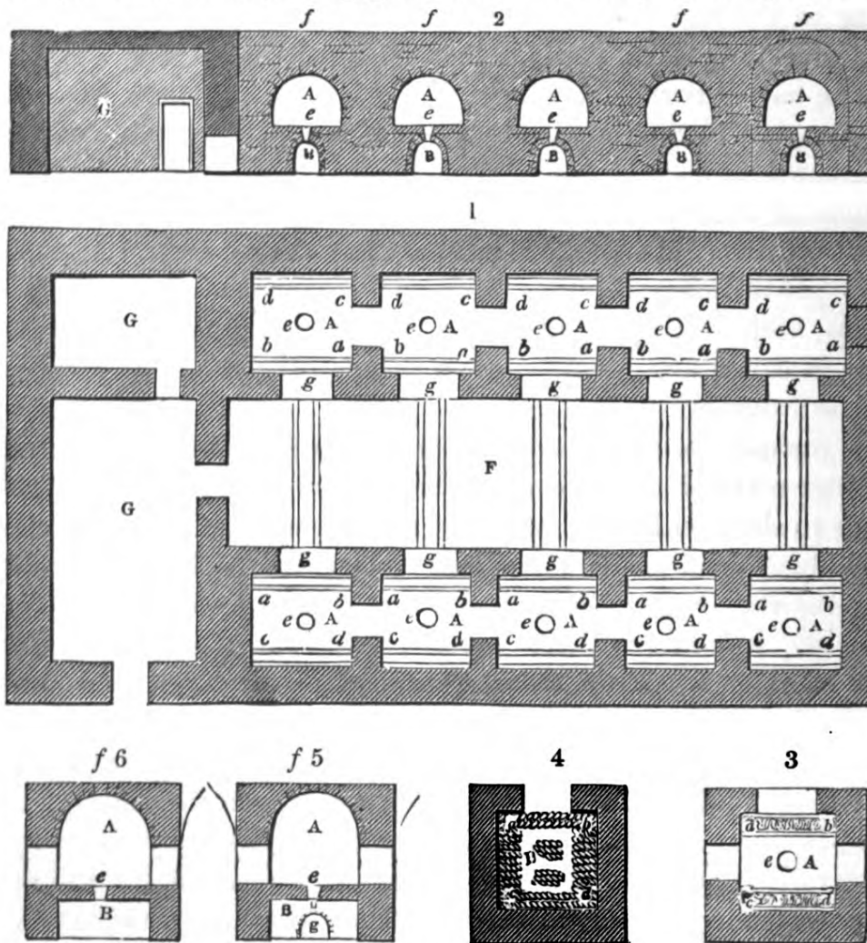
412. Modern ovens for hatching eggs.
