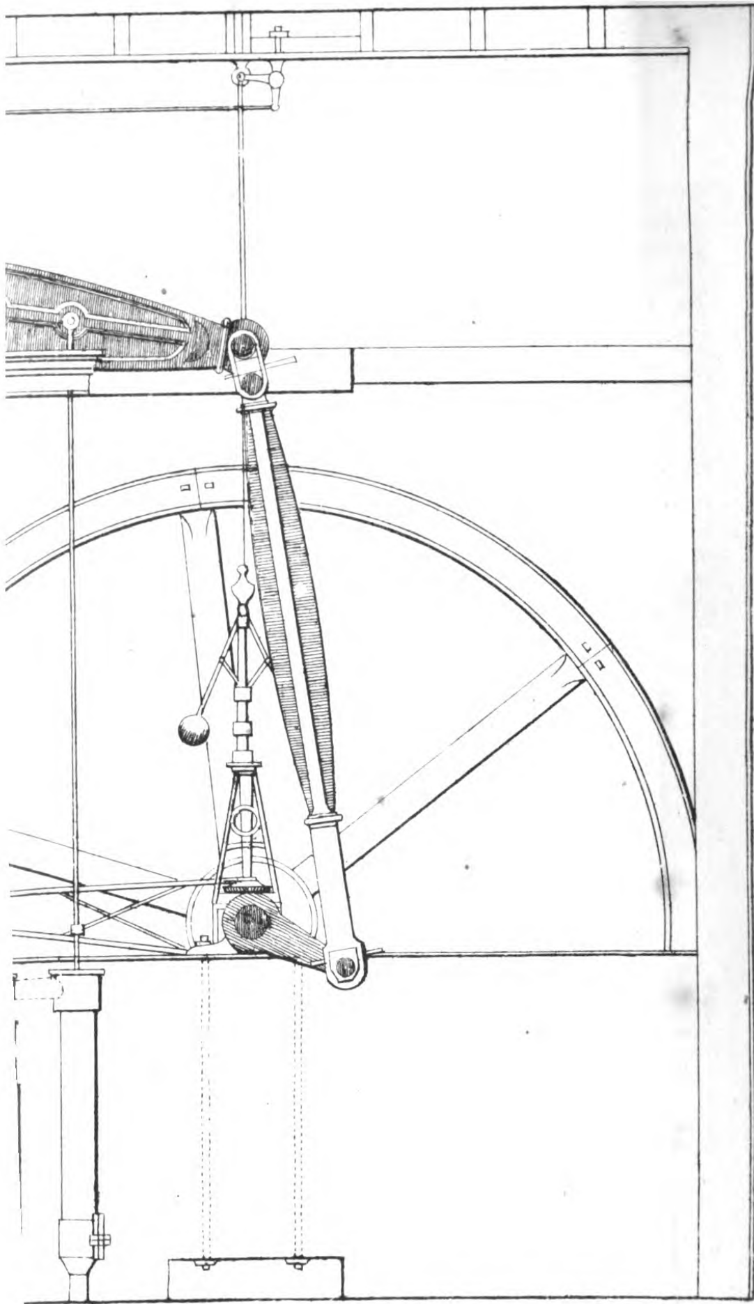
FIG. 10. PRINCIPLE.
