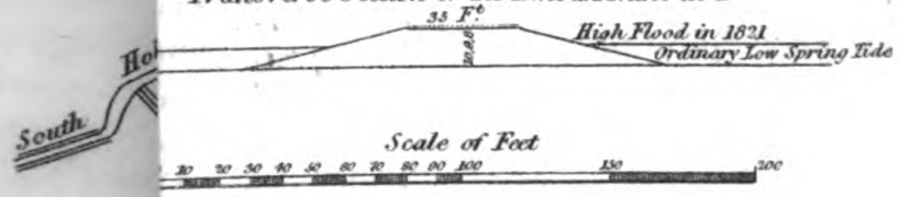
Transverse Section at C
