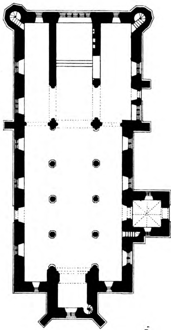
PLAN OF WIMINGTON CHURCH, BEDFORDSHIRE.
