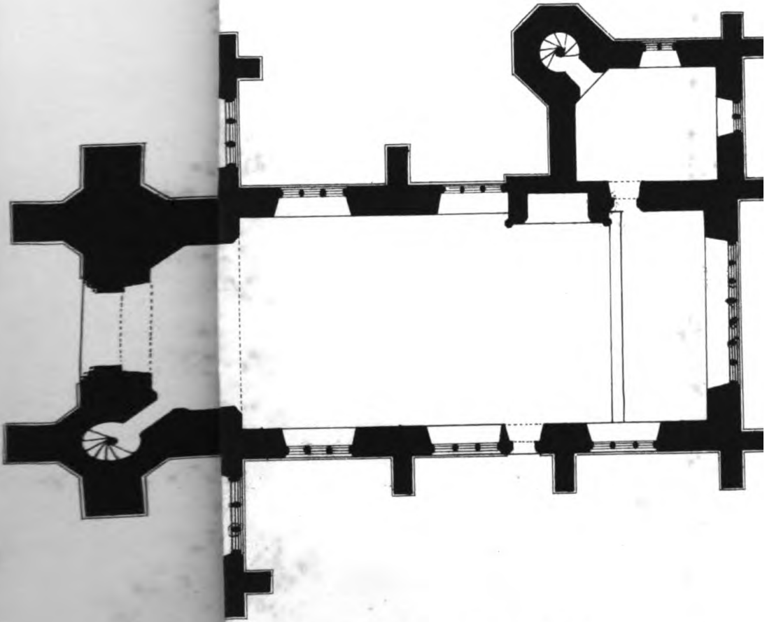
PLAN OF HINGHAM CHURCH, NORFOLK.
