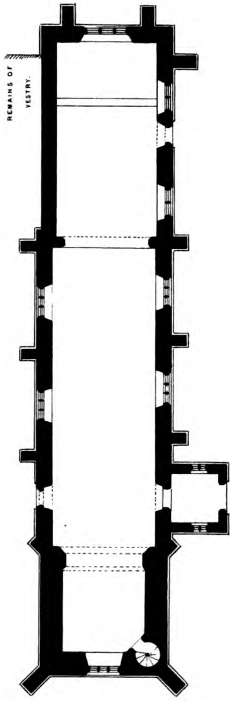
PLAN OF MORLEY ST. BOTOLPH CHURCH, NORFOLK.
