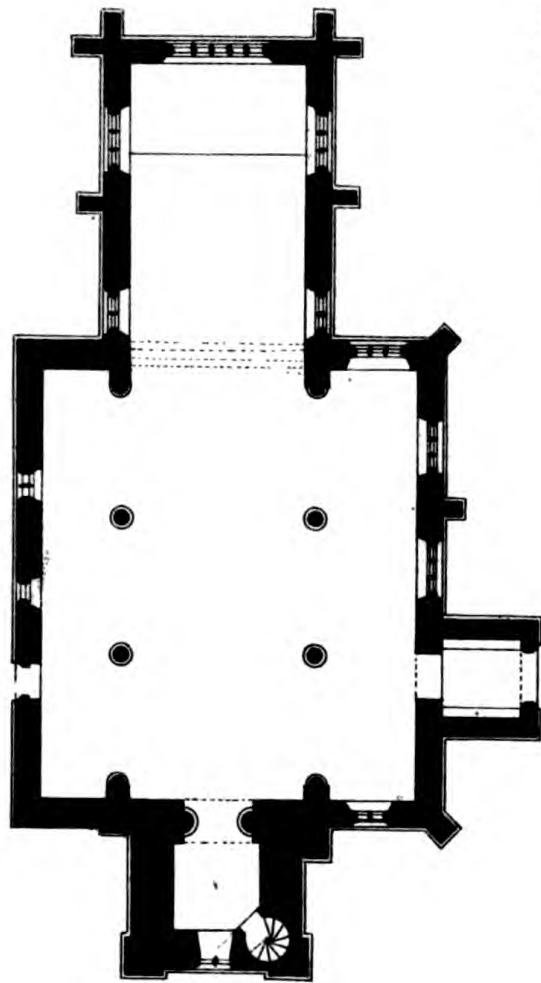
PLAN OF AYSTON CHURCH, RUTLANDSHIRE.
