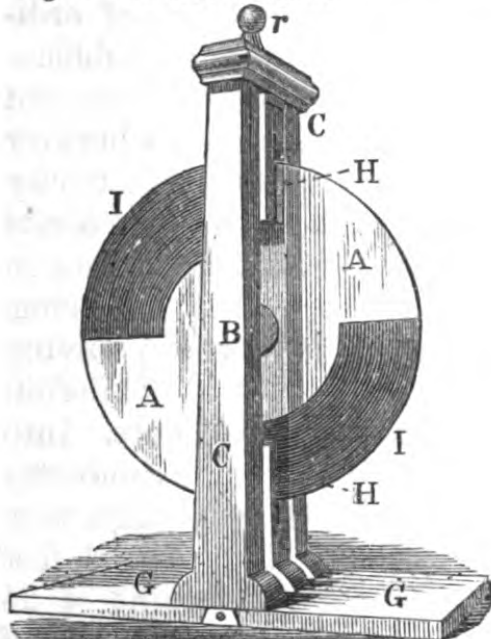
Fig. 78. — PARTS OF PLATE MACHINE.
