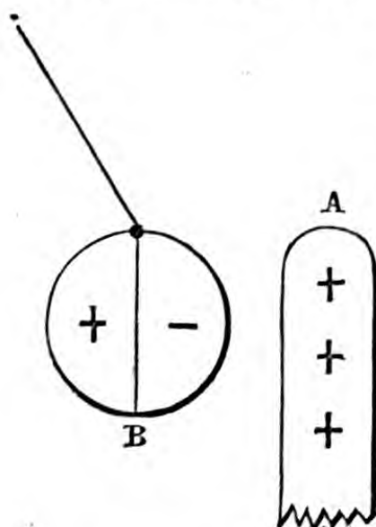
Fig. 66.--SHOWING THAT ATTRACTION IS PRECEDED BY INDUCTION.
