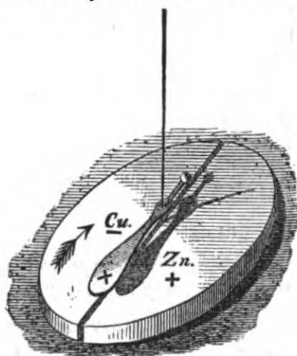
Fig. 144.—SHOWING CHANGE OF ELECTRIC POTENTIAL DUE TO CONTACT OF TWO DISSIMILAR METALS. Consists of a semicircular disc of copper in contact with a similar disc of zinc, above which is suspended, by means of a fine wire from the interior of a positively charged Leyden jar, a light aluminium needle.
