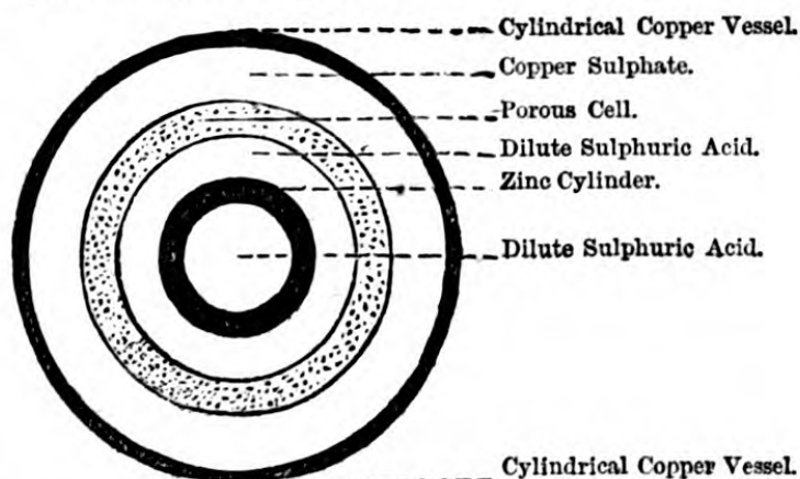
Fig. 128.—HORIZONTAL SECTION OF A CHARGED DANIELL'S ELEMENT.
