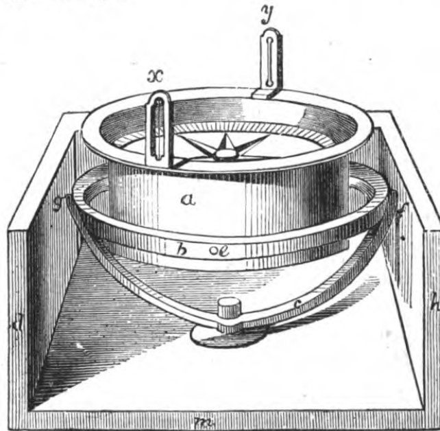
Fig. 34. — MARINER'S COMPASS. a , Compass box containing compass needle and floating card; b, c , gimbals; d, h, m , external wooden case; e , one of the pivots on which compass case swings; f, g , pivots on which horizontal gimbal swings; x, y , sight vanes sometimes attached to magnetic compasses, especially land compasses.
