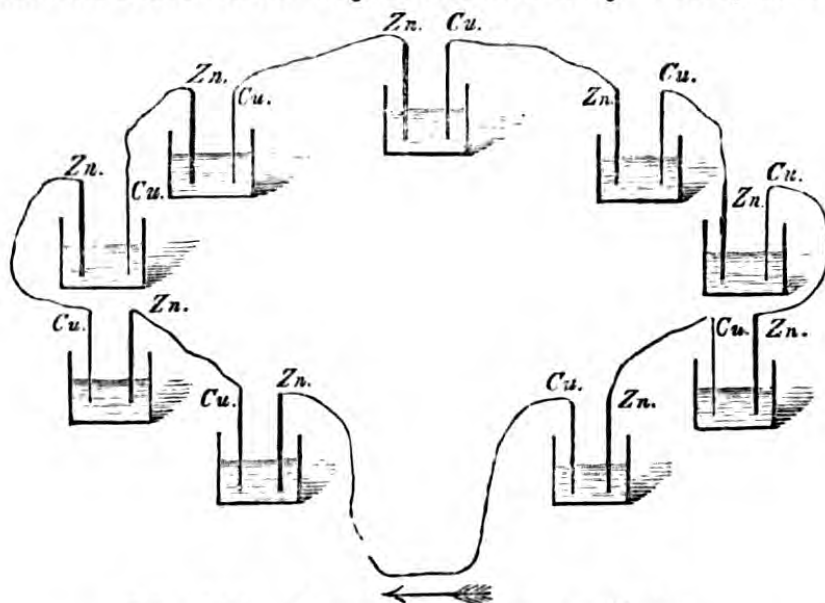
Fig. 124.—VOLTA'S CROWN OF CUPS.
