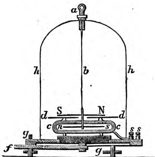
Fig. 139.—ASTATIC GALVANOMETER OR MULTIPLIER (Vertical Section).
