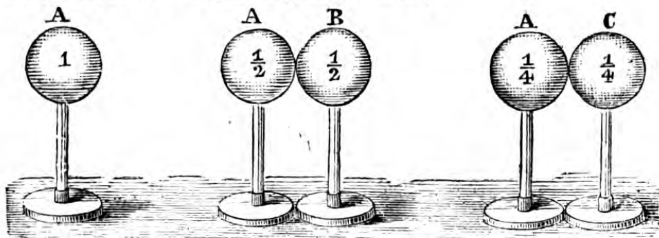
Fig. 84.—SHOWING DIVISION OF ELECTRIC CHARGE.
