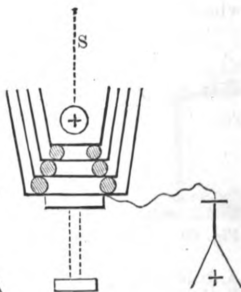
Fig. 62. — FARADAY'S FOUR ICE PAILS EXPERIMENT.
