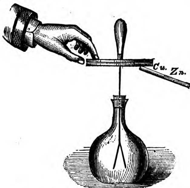
Fig. 142.—VOLTA'S EXPERIMENT.
