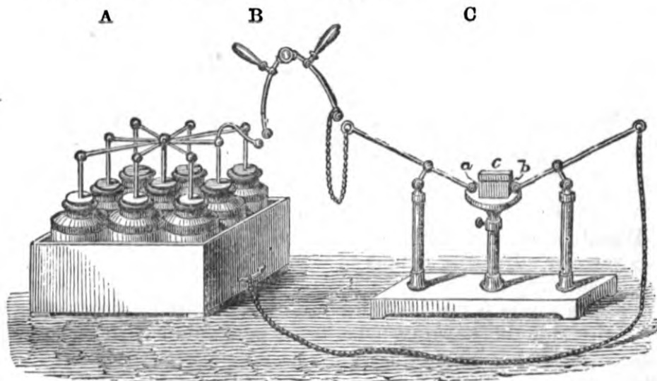
Fig. 102.—SHOWING MODE OF DISCHARGING LEYDEN BATTERY THROUGH GLASS OR OTHER REFRACTORY SUBSTANCE.
