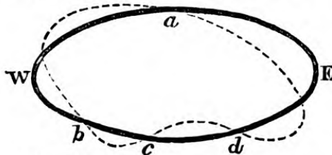
Fig. 38.—GEOGRAPHICAL AND MAGNETIC EQUATOR
