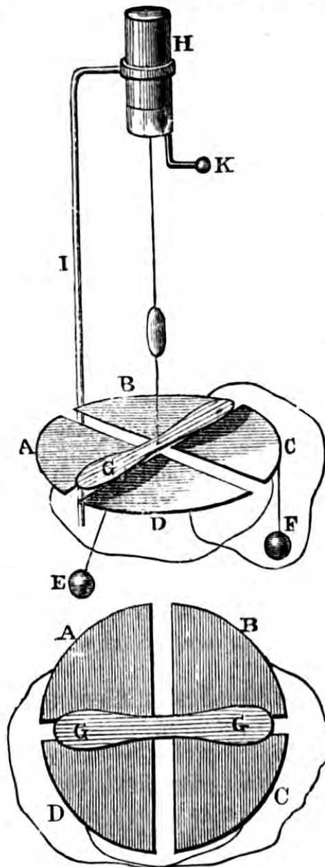
Fig. 98.—SIR WILLIAM THOMSON'S QUADRANT ELECTROMETER.
