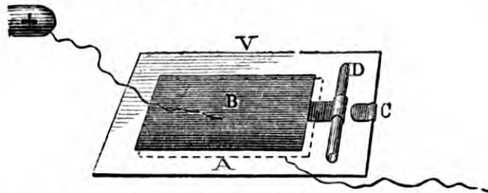
Fig. 96.—SHOWING MODE OF CHARGING FULMINATING PANE.
