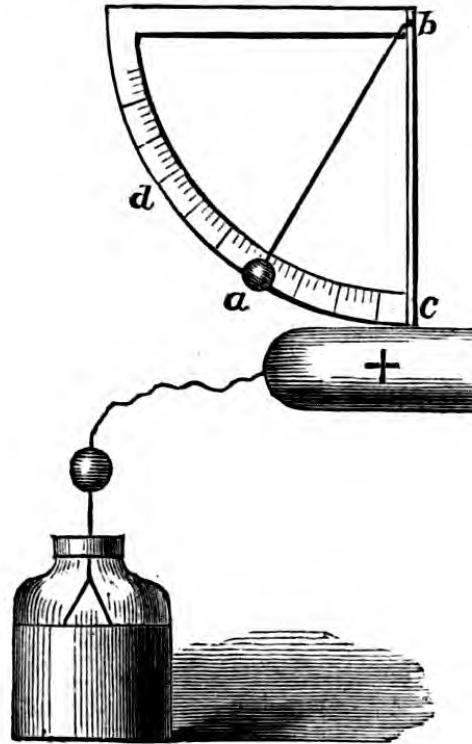
Fig. 55.—MEASURING ELECTRIC TENSION BY QUADRANT ELECTROMETER.
