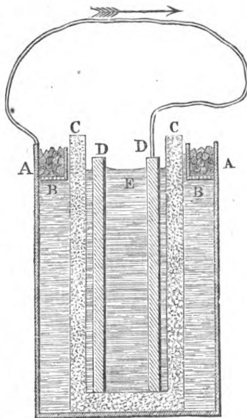
Fig. 127.—VERTICAL SECTION OF A CHARGED DANIELL'S ELEMENT.
