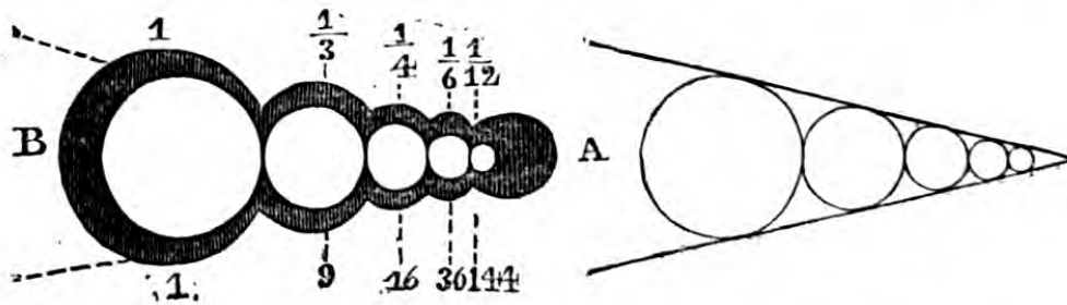
Fig. 93.—ILLUSTRATES THEORY OF THE ACTION OF POINTS CONSIDERED AS A SUCCESSION OF GRADUALLY DIMINISHING SPHERES.
