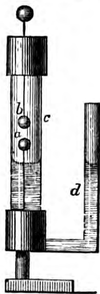
Fig. 110.—KINNERSLEY'S (ELECTRIC) THERMOMETER.
