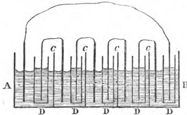
Fig. 132.—DANIELL'S BATTERY AS ARRANGED IN TELEGRAPHY.
