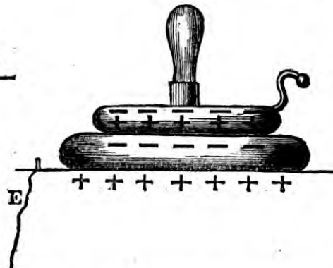
Fig. 69.—SHOWING DECOMPOSITION OF NEUTRAL ELECTRICITY IN COLLECTING PLATE, by inductive action of vulcanite or generating plate.
