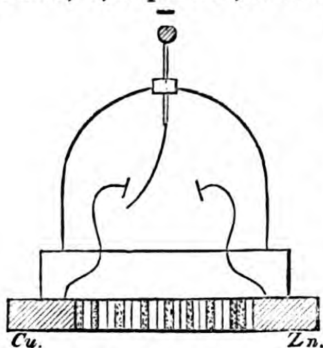
Fig. 125.—BOHNENBERGER'S ELECTROSCOPE.
