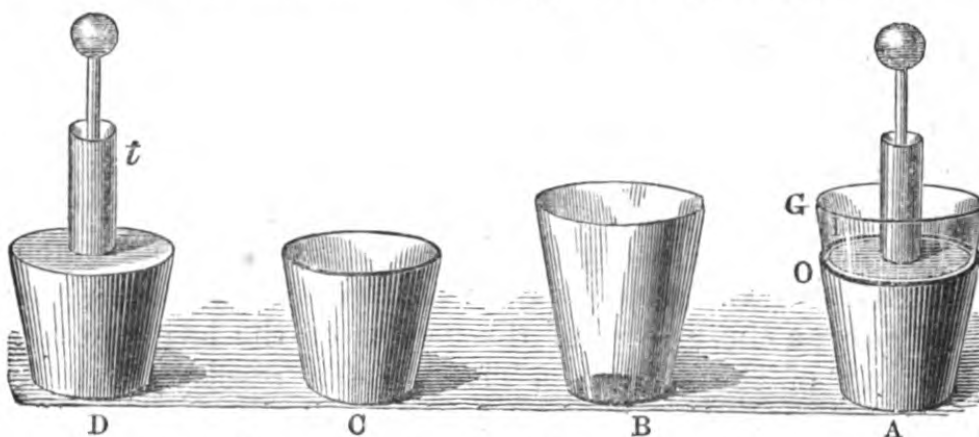
Fig. 105.—DISSECTED LEYDEN JAR WITH MOVABLE TIN COATINGS.
