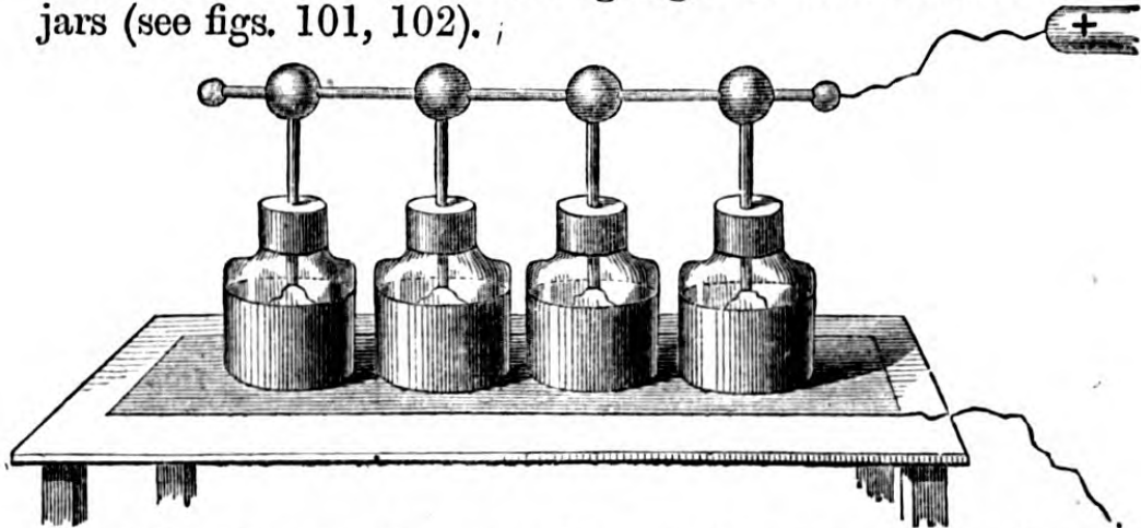
Fig. 101.—MODE OF CHARGING LEYDEN BATTERY OF FOUR JARS.
