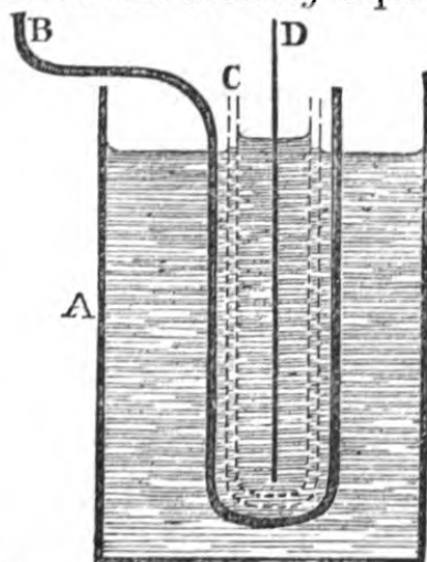
Fig. 129.—VERTICAL SECTION OF A GROVE'S CELL.
