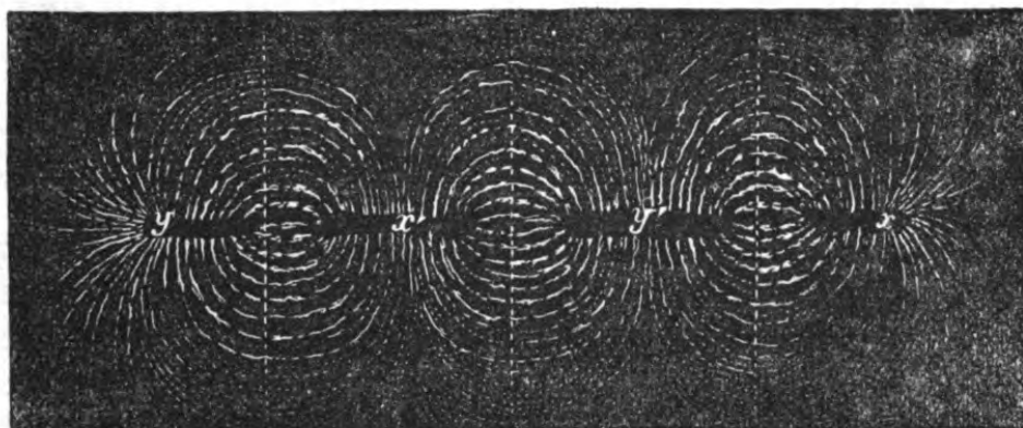
Fig. 24.—BAR MAGNET, WITH IRON FILINGS about consequent points. x , y , North and South Poles; x' , y' , consequent points. The dotted straight lines show neutral lines or Magnetic Equators .
