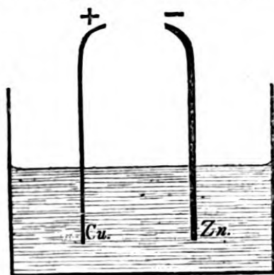
Fig. 120.—ILLUSTRATING THE ORDINARY THEORY OF ELECTRIC CONDITION OF PLATES OF COPPER AND ZINC BEFORE METALLIC CONTACT.
