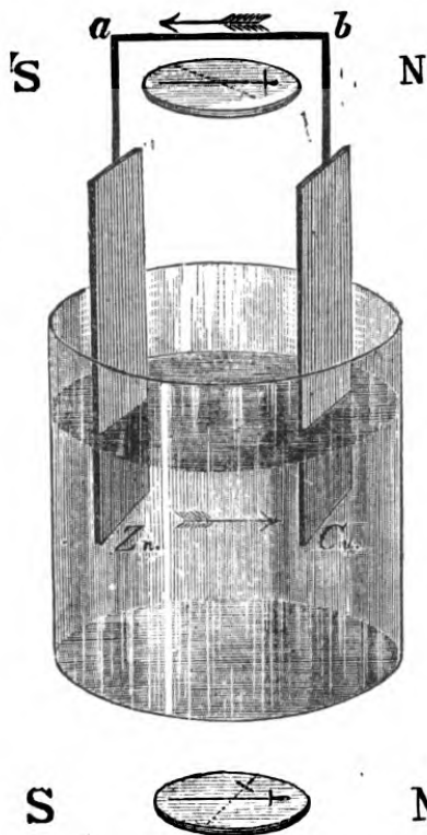
Fig. 136.—SHOWING DIRECTION IN WHICH COMPASS NEEDLE IS DEFLECTED BY VOLTAIC CURRENT PASSING ABOVE AND BELOW NEEDLE.
