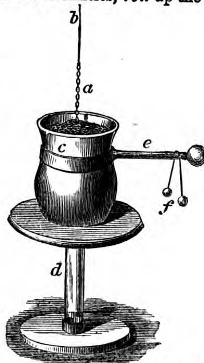
Fig. 88.—METALLIC CHAIN APPARATUS FOR ILLUSTRATING ELECTRIC DENSITY.
