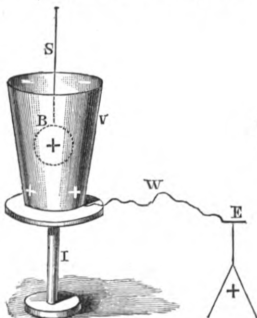
Fig. 61. — FARADAY'S ICE PAIL EXPERIMENT.
