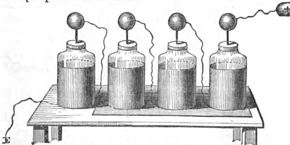
Fig. 103.—ARRANGEMENT FOR CHARGING LEYDEN BATTERY BY CASCADE.
