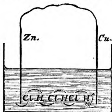
Fig. 140.—SHOWING POLARIZATION OF MOLECULES OF HYDROCHLORIC ACID IN WORKING VOLTAIC CELL.
