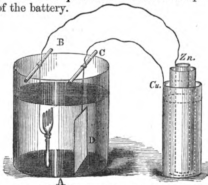
Fig. 145.—ELECTRO-PLATING APPARATUS.
