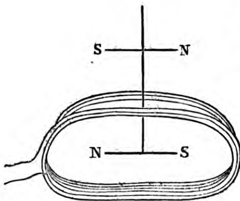
Fig. 138.—ASTATIC NEEDLE.
