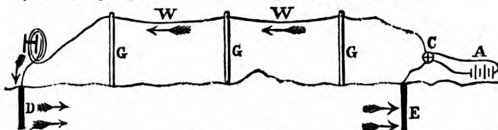
Fig. 148.—SHOWING GENERAL ARRANGEMENT OF TELEGRAPH AND LINE.
