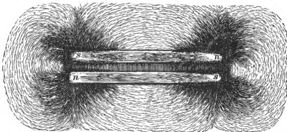
Fig. 20.—IRON FILINGS, showing lines of force about two parallel Bar Magnets, with their contrary poles adjacent.
