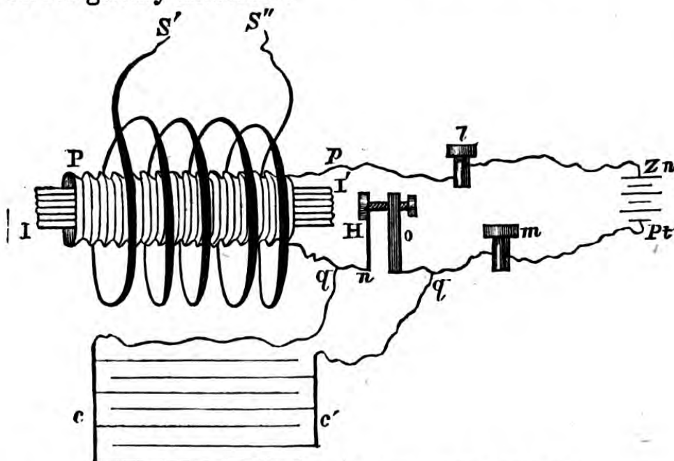
Fig. 151.—DISSECTED RUHKORFF'S COIL.
