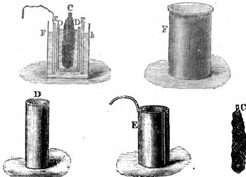
Fig. 131.—VERTICAL SECTION OF A BUNSEN'S CELL.
