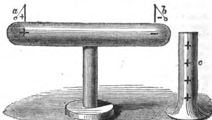
Fig. 59.—SHOWING INDUCTIVE ACTION OF RUBBED GLASS PILLAR ON NEUTRAL METAL CYLINDER MOUNTED ON GLASS LEG.
