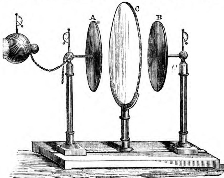
Fig. 94.—ÆPINUS'S CONDENSER.
