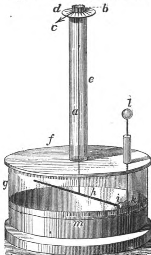
Fig. 56.—COULOMB'S TORSION ELECTROMETER.
