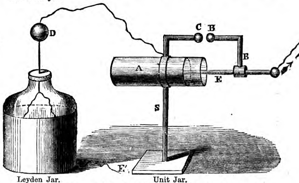
Fig. 104.—SHOWING MODE OF MEASURING CHARGE OF LEYDEN JAR BY MEANS OF HARRIS'S UNIT JAR (A).
