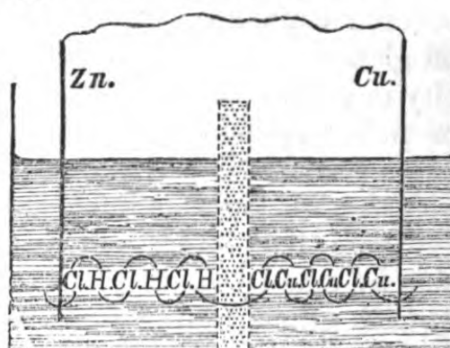
Fig. 141.—SHOWING PROPAGATION OF STATE OF POLARIZATION FROM MOLECULES OF HYDROCHLORIC ACID THROUGH POROUS DIAPHRAGM TO MOLECULES OF CUPROUS CHLORIDE.
