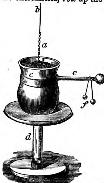
Fig. 88.—METALLIC CHAIN APPARATUS FOR ILLUSTRATING ELECTRIC DENSITY.
