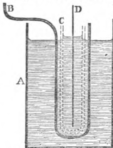
Fig. 114.—VERTICAL SECTION OF A GROVE'S CELL.
