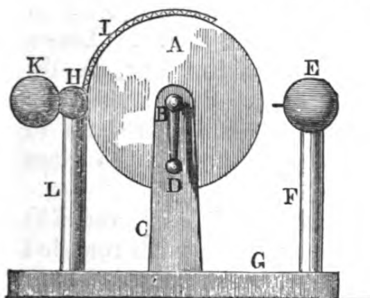
Fig. 72. — VERTICAL PLAN OF CYLINDRICAL MACHINE, seen endwise.
