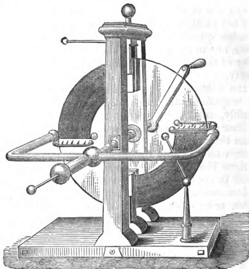
Fig. 77.—COMMON PLATE ELECTRICAL MACHINE.
