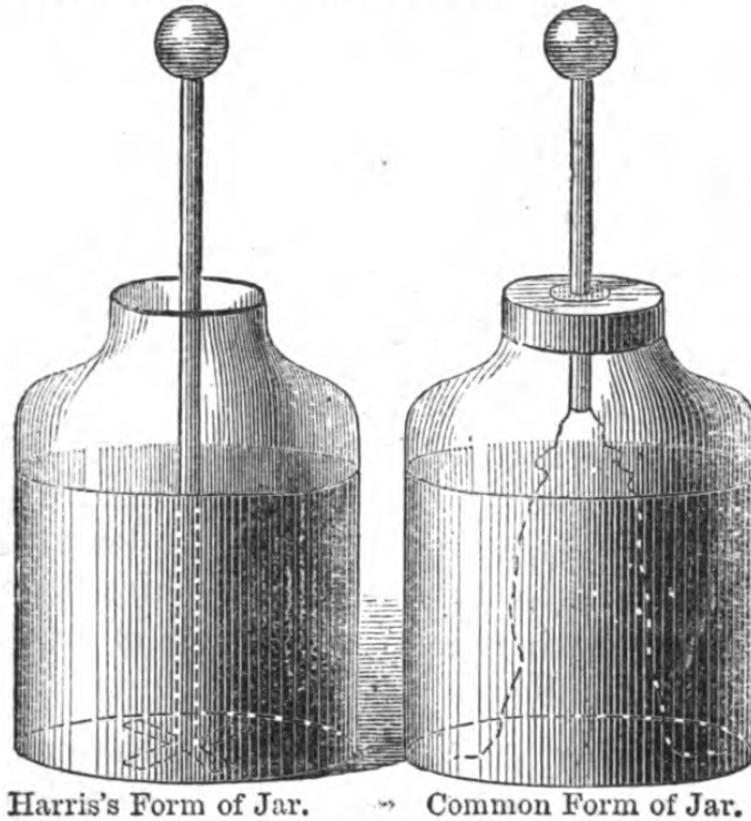
Fig. 94.—LEYDEN JARS.
