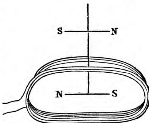
Fig. 119.—ASTATIC NEEDLE.
