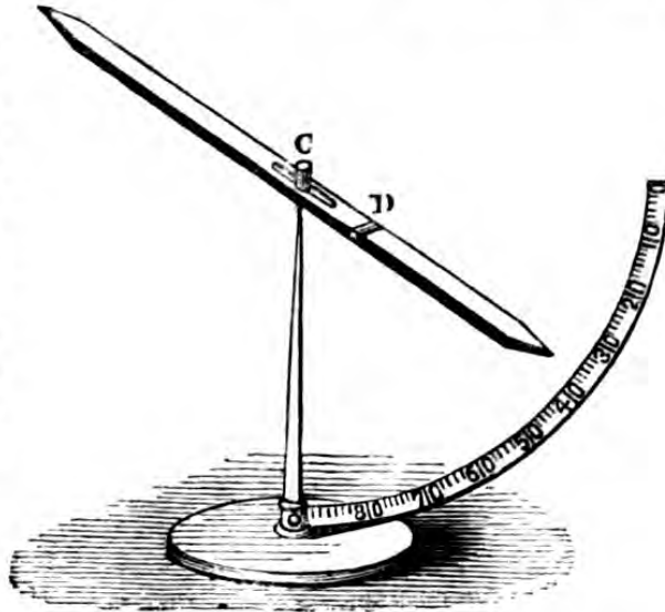
Fig. 36. — SIMPLE FORM OF DIPPING NEEDLE. C, Agate cap; D, north or dipping end of Needle.
