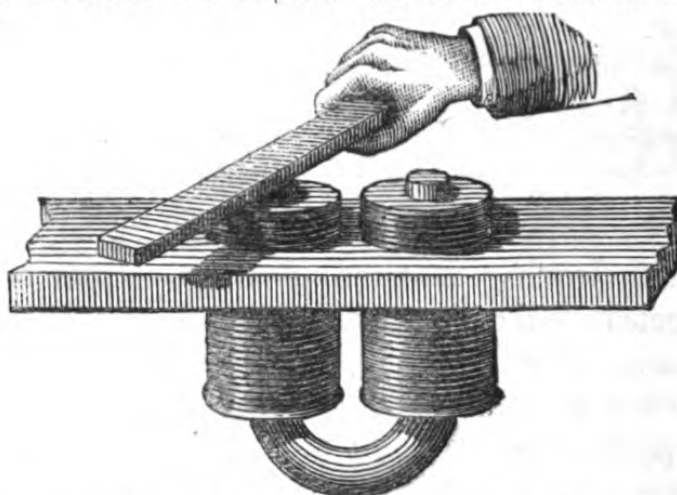
Fig. 18.—METHOD OF MAGNETIZATION BY AN ELECTRO-MAGNET.
