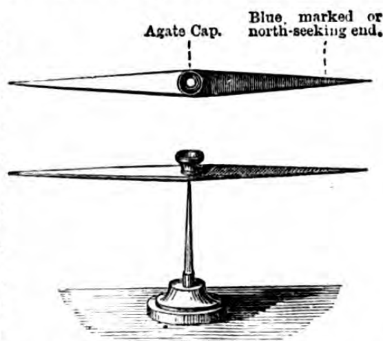
Fig. 33. — MAGNETISED COMPASS NEEDLE Mounted on vertical steel point.
