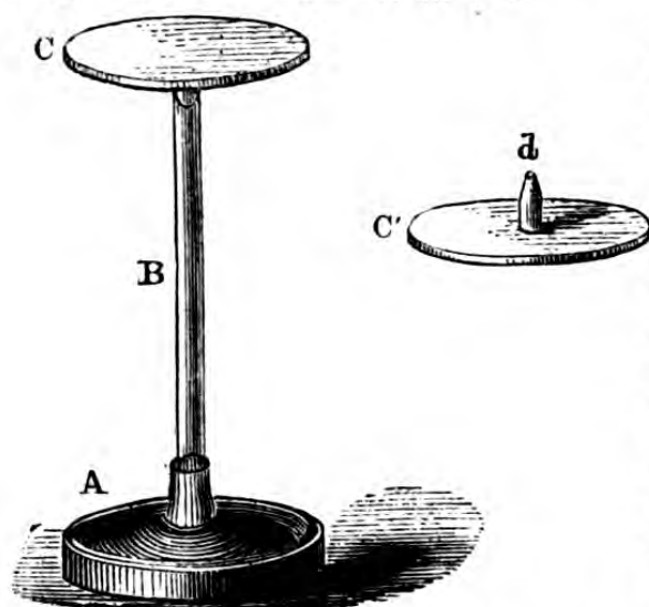
Fig. 47.—INSULATING STAND.
