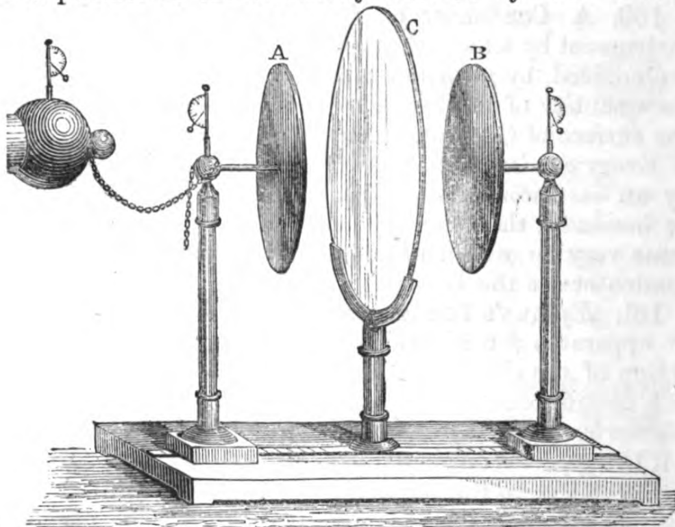
Fig. 92.—ÆPINUS'S CONDENSER.
