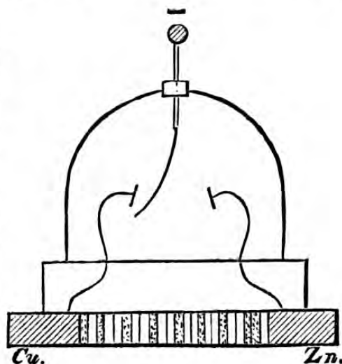
Fig. 111.—BOHNENBERGER'S ELECTROSCOPE.
