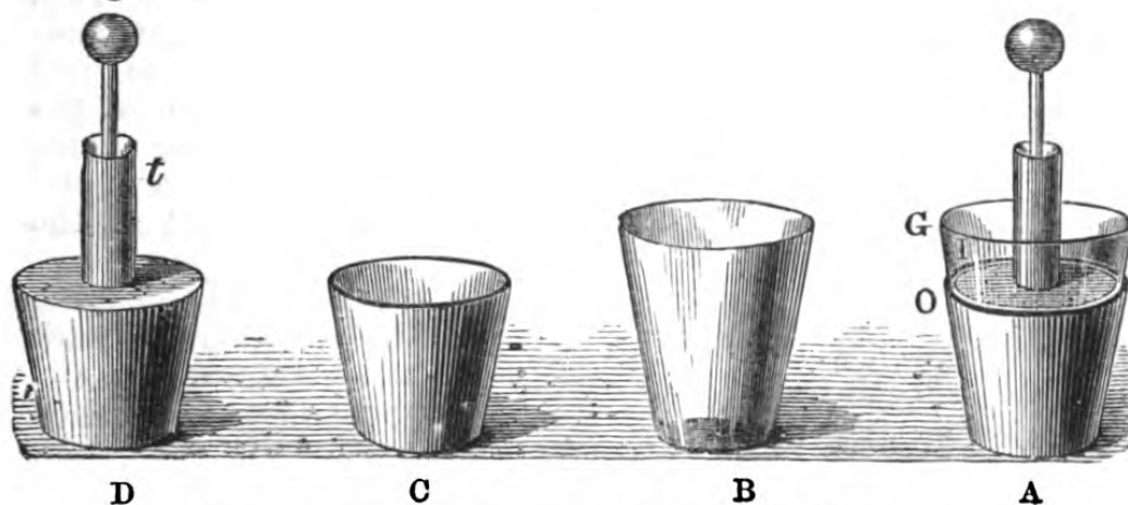
Fig. 97.—DISSECTED LEYDEN JAR WITH MOVABLE TIN COATINGS.
