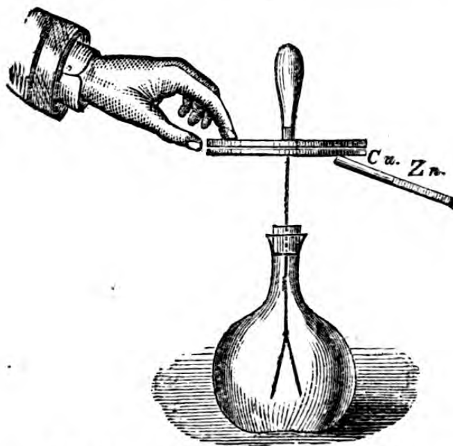
Fig. 116.—VOLTA'S EXPERIMENT.
