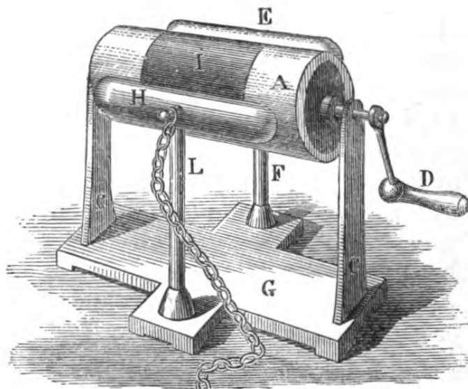
Fig. 71.—CYLINDRICAL ELECTRICAL MACHINE.
