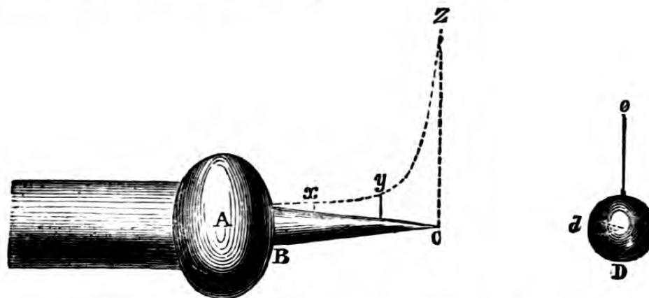
Fig. 91.—SHOWING ELECTRIC DENSITY AT POINTS.
