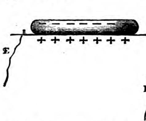
Fig. 68.—SHOWING VULCANITE CAKE CHARGED WITH NEGATIVE ELECTRICITY, resting on Metallic Plate or sole in connection with the earth .
