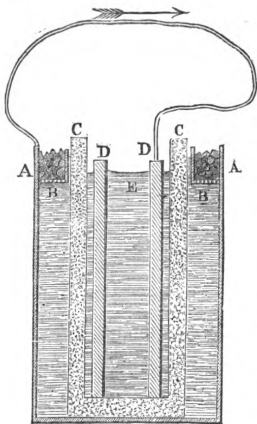
Fig. 113.—VERTICAL SECTION OF A CHARGED DANIELL'S ELEMENT.
