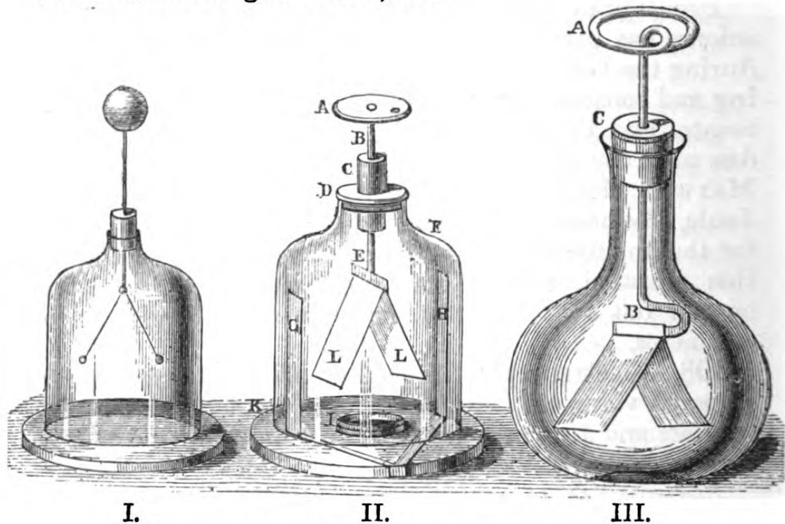
Fig. 49.—ELECTROSCOPES.
