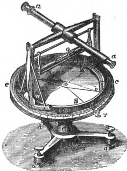
Fig. 32. — DECLINATION COMPASS. a, a , Telescope; b, b , compass box and needle; c, c , horizontal limb (graduated); d, d, d , tripod with levelling screws; e , pillar in which graduated limb rotates.
