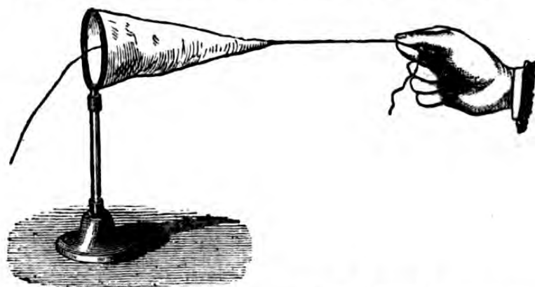
Fig. 85.—FARADAY'S BUTTERFLY NET EXPERIMENT.
