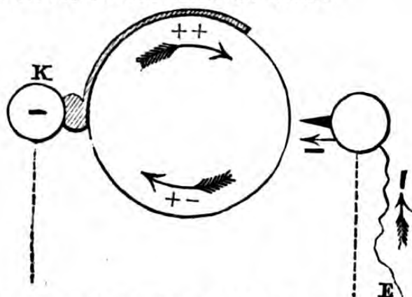
Fig. 75. — SHOWING PASSAGE OF NEGATIVE ELECTRICITY from the earth , through the wire (E) to the prime conductor, thence to the glass cylinder, and thence to the rubber (K). The rubber in this case is supposed to be insulated , and the prime conductor connected with the earth , as when charging bodies with negative electricity.
