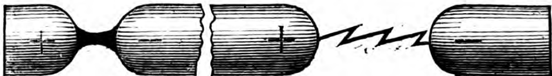
Fig. 102.—STRAIGHT AND ZIG-ZAG ELECTRIC SPARKS.
