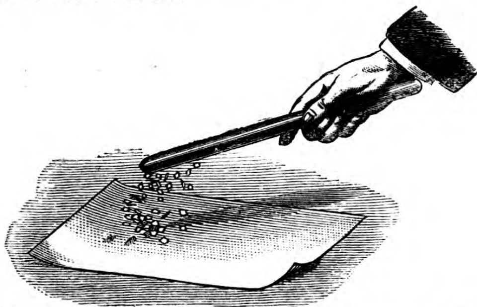
Fig. 39. — SHOWING ATTRACTION AND REPULSION OF LIGHT BODIES, as feathers (down), chopped straw or paper, bran, sawdust, gold-leaf, and pith balls, by warm rubbed rod of vulcanite, sealing-wax, or glass.
