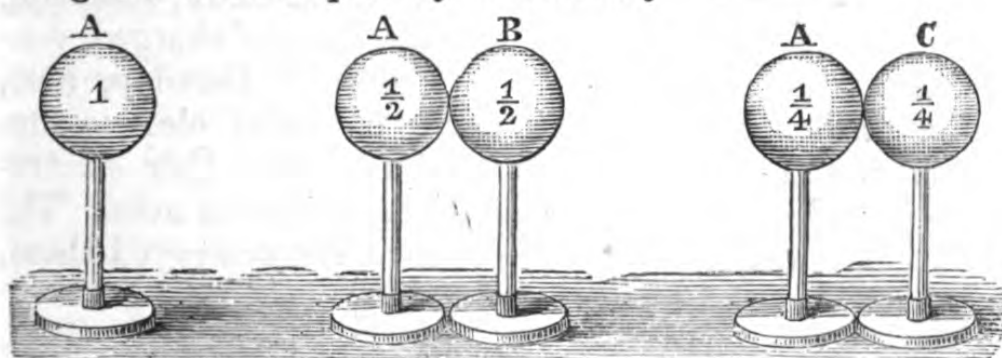
Fig. 84.—SHOWING DIVISION OF ELECTRIC CHARGE.
