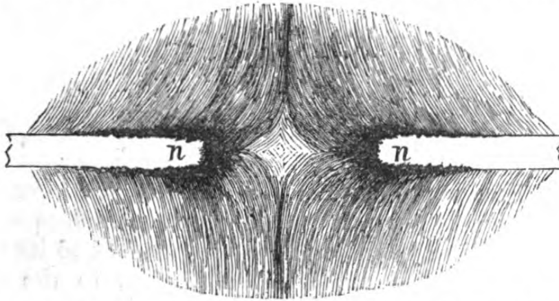
Fig. 23.—IRON FILINGS, showing lines of magnetic force about the two similar Poles of two Bar Magnets, placed end to end .
