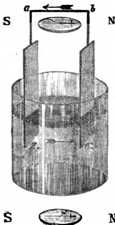
Fig. 117.—SHOWING DIRECTION IN WHICH COMPASS NEEDLE IS DEFLECTED BY VOLTAIC CURRENT PASSING ABOVE AND BELOW NEEDLE.
