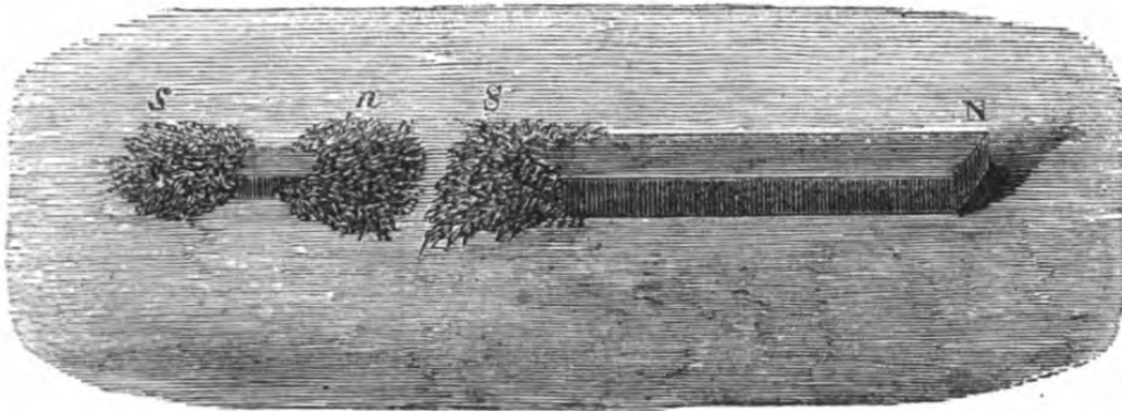
Fig. 26.—SHOWING MAGNETIC INDUCTION. N, S, North and South Poles of a Bar Magnet. n, s, North and South Poles of a piece of soft iron magnetised inductively (at a distance) by the permanent bar magnet. The magnetised state of the soft iron bar is shown by the adhesion of the iron filings.
