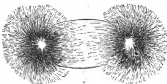
Fig. 2.—Showing IRON FILINGS clustered about the poles of a natural magnet or loadstone.
