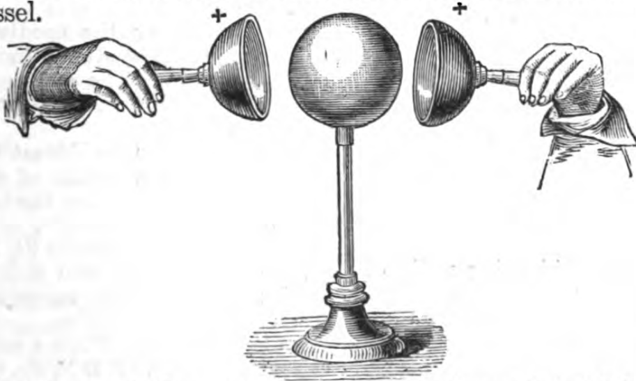
Fig. 81.—BIOT'S EXPERIMENT, showing tendency of electricity in insulated ball to escape to outer surface of insulated hemispherical caps.
