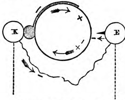
Fig. 76.—SHOWING PASSAGE OF NEGATIVE ELECTRICITY from the positive or prime conductor (E) to the glass cylinder, thence to the rubber (K), and back again to the prime conductor.—In this case the prime conductor and the rubber are supposed to be connected.
