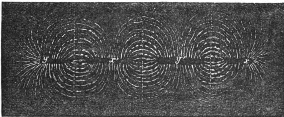
Fig. 24.—BAR MAGNET, WITH IRON FILINGS about consequent points. x , y , North and South Poles ; x' , y' , consequent points. The dotted straight lines show neutral lines or Magnetic Equators .
