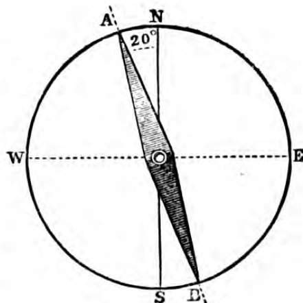
Fig. 31. — COMPASS NEEDLE, SHOWING DECLINATION of 20^{\circ} W.
