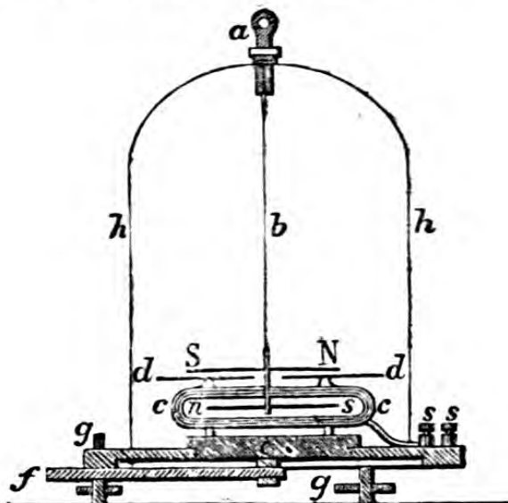
Fig. 120.—ASTATIC GALVANOMETER OR MULTIPLIER (Vertical Section).
