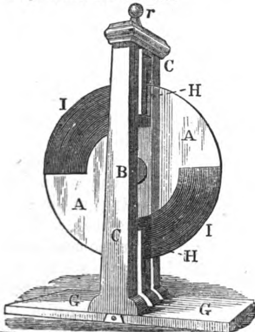
Fig. 78. — PARTS OF PLATE MACHINE.
