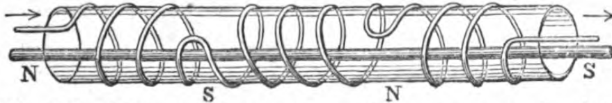
Fig. 16.—MIXED HELIX, arranged for consequent points.
