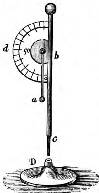
Fig. 54.—HENLEY'S QUADRANT ELECTROMETER.
