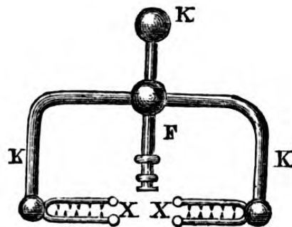
Fig. 79. — PRIME CONDUCTOR OF PLATE MACHINE.
