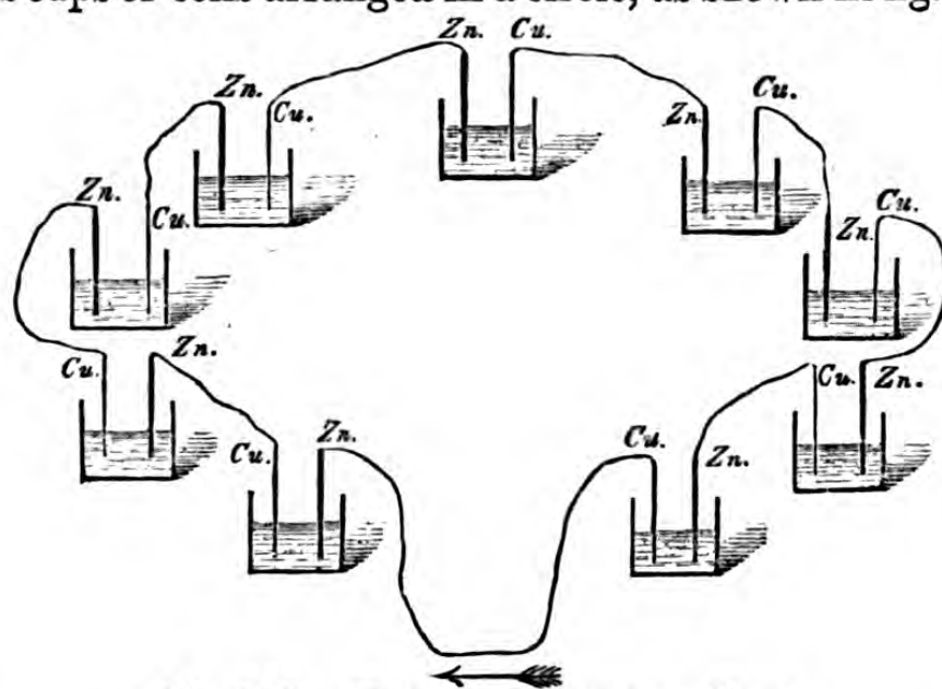
Fig. 110.—VOLTA'S CROWN OF CUPS.
