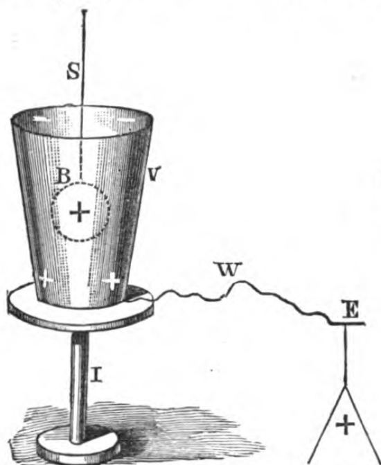
Fig. 61. — FARADAY'S ICE PAIL EXPERIMENT.
