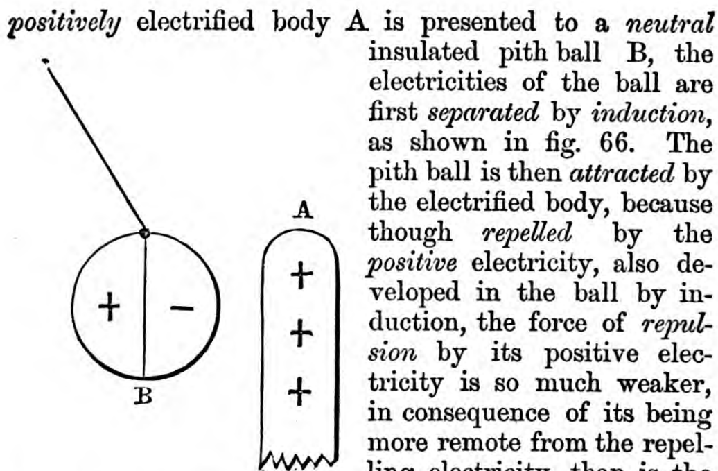
Fig. 66. --SHOWING THAT ATTRACTION IS PRECEDED BY INDUCTION.
