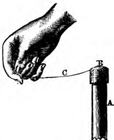
Fig. 48.—Simple Apparatus for proving that EQUAL QUANTITIES OF THE TWO KINDS OF ELECTRICITY ARE DEVELOPED AT THE SAME TIME.
