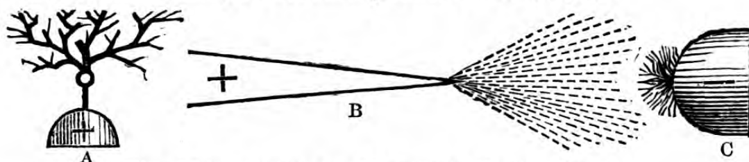
Fig. 104.—SHOWING ELECTRIC GLOW, BRUSH.
