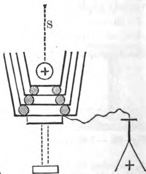
Fig. 62. — FARADAY'S FOUR ICE PAILS EXPERIMENT.
