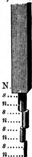
Fig. 3.—MAGNETIC CHAIN, consisting of a bar magnet and a series of pieces of soft iron adhering together, under the influence of magnetic induction.
