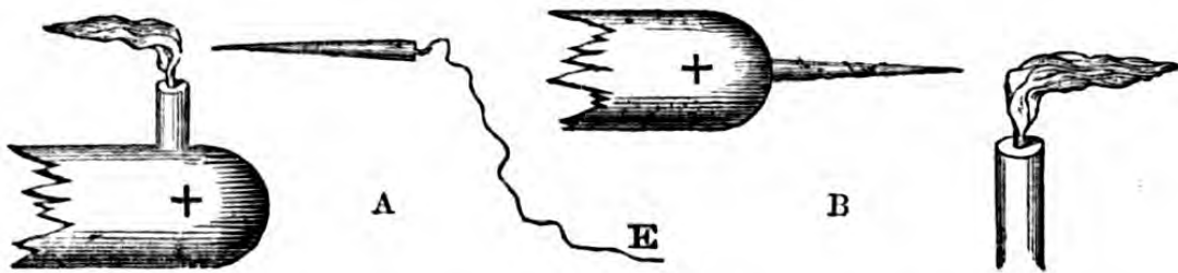
Fig. 101.—SHOWING ACTION OF POINTS ON FLAME.
